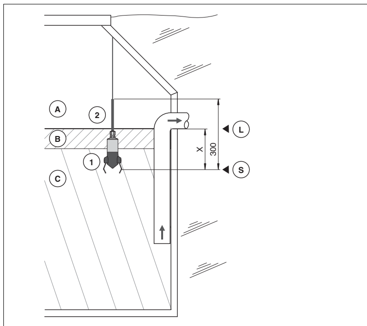
Figure 3.2 Mounting the fat level sensor
