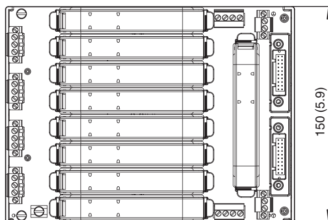
Figure 2.4_Dimensions Motherboard MBHD-FB-D-4R.YO
