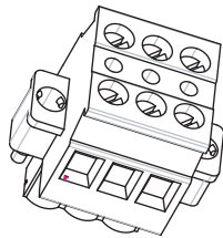
Figure 3.5 T-connector for Trunk and Terminator connection
