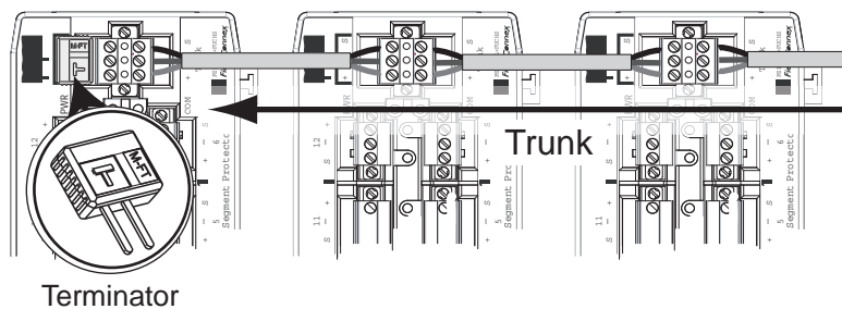
Figure 3.6 Stylized series connection and termination
