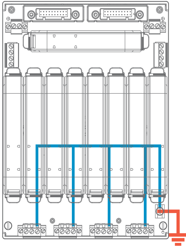
Figure 3.1 Internal connections between trunk connectors and ground connection clamp
