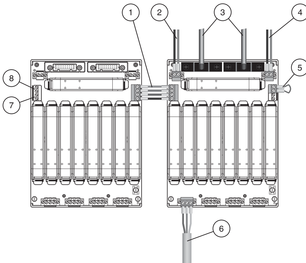
Figure 3.2Connections of the motherboard
