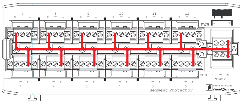
Figure 3.4 Stylized composition of the shield lines within the Segment Protector
