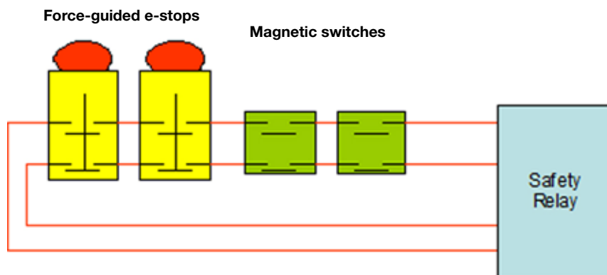
Figure 1: Magnetic REED safety switches (green devices) and safety e-stops (yellow/red devices) are switched in series and connected to the inputs on a safety relay. If one of the safety switches fails with a welded contact, it is still possible to restart the machine by cycling any of the other safety switches. Consequently, the machine will start up even though it is in a state of reduced redundancy. A second failure on the same partially-failed safety device would make the safety function entirely unavailable; certainly not a very good situation.
