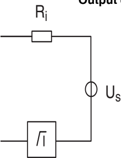
Output circuit diagram
