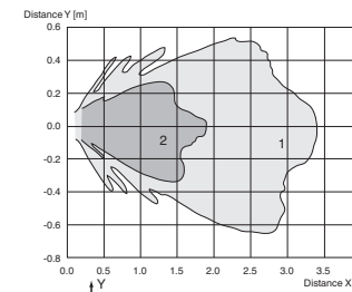
Kurve 1: flat surface 100 mm x 100 mm Kurve 2: round bar, Ø 25 mm
