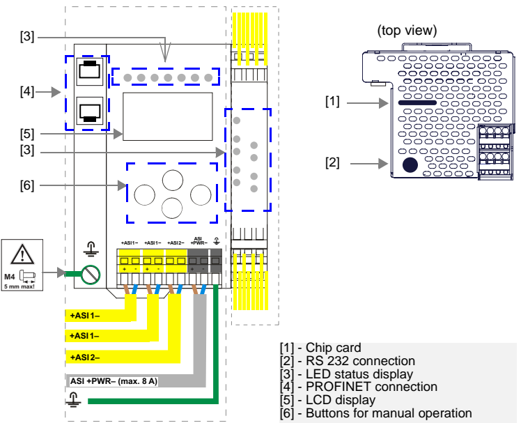
Fig. 1 Gateway connection diagram
