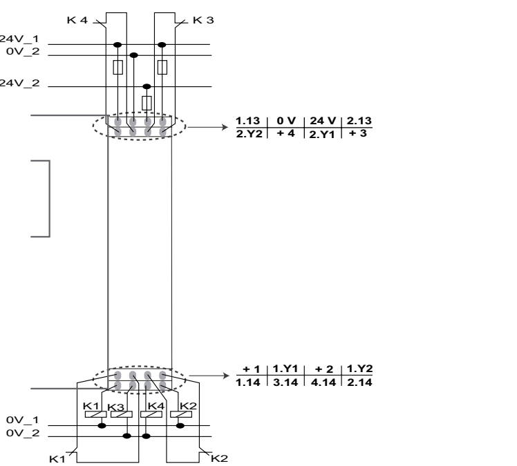
Fig. 2: Safety unit connection diagram
