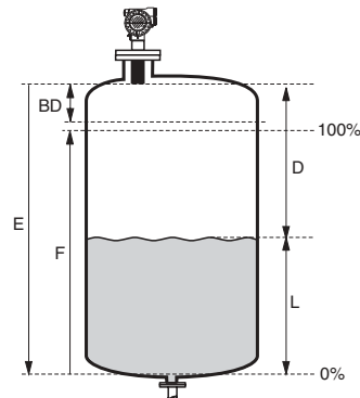
BD: Blockdistanz
