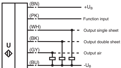
Fig. 7.1: Electrical connection
