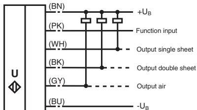
Fig. 7.1: Electrical connection of device versions ...-3E0 and ...-3E1
