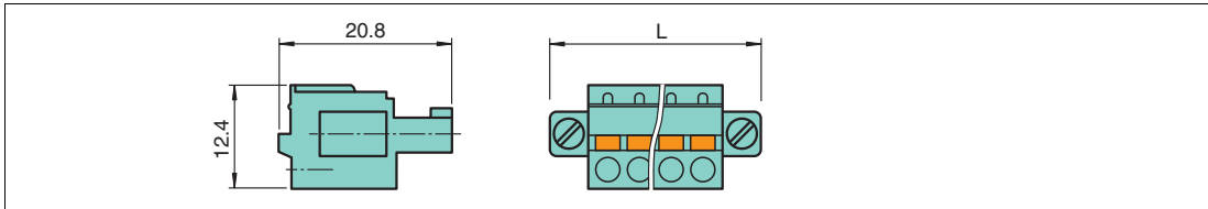
Figure 2.18 Spring terminal dimensions L = 33.3 mm for 6-pin terminal and 40.9 mm for 8-pin terminal
