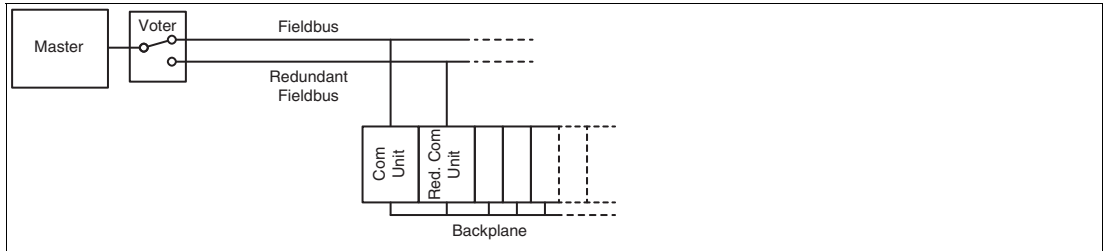
Figure 3.14 Line redundancy
