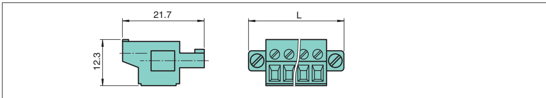
Figure 2.17 Front screw terminal dimensions L = 33.3 mm for 6-pin terminal and 40.9 mm for 8-pin terminal
