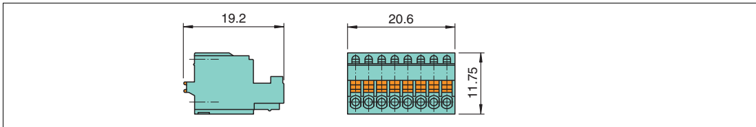
Figure 2.19 Spring terminal dimensions
