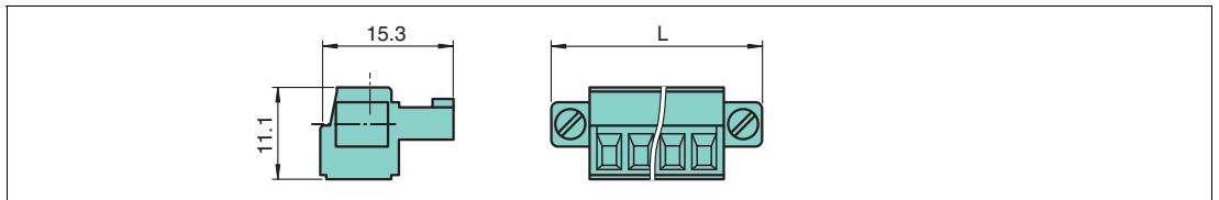
Figure 2.16 Screw terminal dimensions L = 33.3 mm for 6-pin terminal and 40.9 mm for 8-pin terminal
