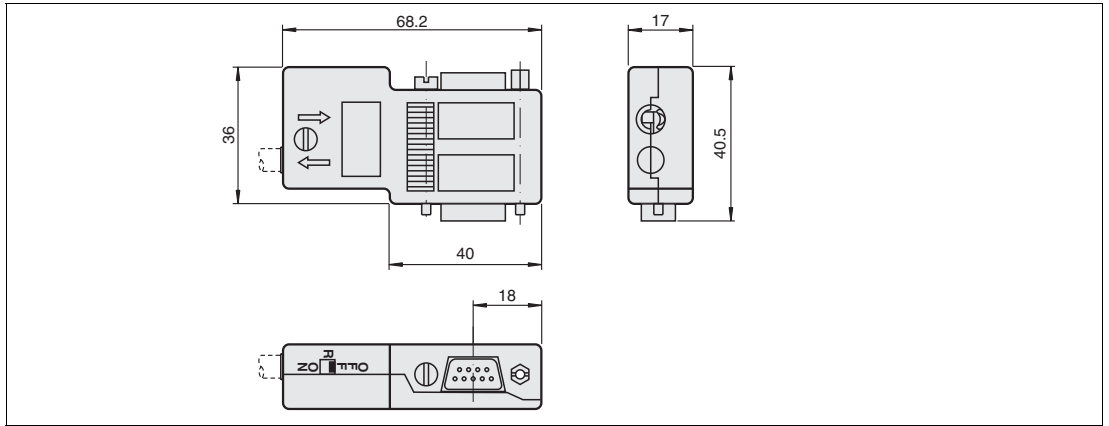
Figure 2.15 Dimensions of the LB9003A
