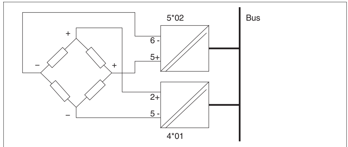
Figure 3.13 Example of a strain gauge bridge
