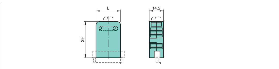
Figure 2.20 Protective cover dimensions L = 25.25 mm for protective covers for 6-pin terminals and 32.87 mm for protective covers for 8-pin terminals
