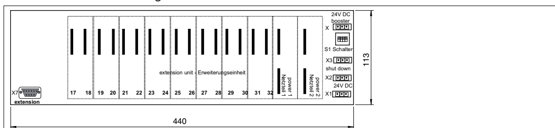
Figure 2.7 Dimensions of the LB9027BP16200.1
