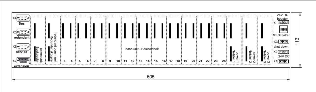
Figure 2.2 Dimensions of the LB9022BP22320.1
