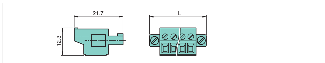
Figure 2.17 Front screw terminal dimensions L = 33.3 mm for 6-pin terminal and 40.9 mm for 8-pin terminal
