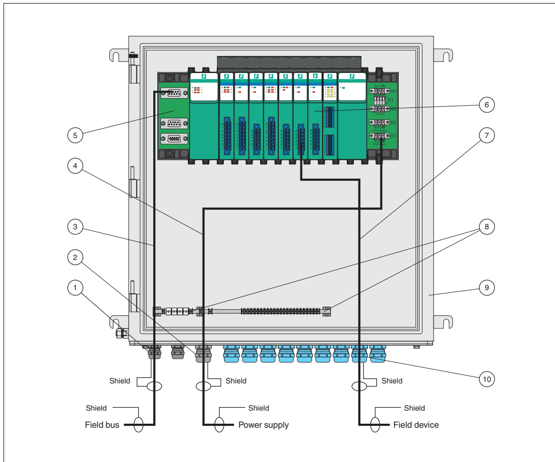
Figure 3.27 Shielding concept in the metal surrounding enclosure for offshore applications
