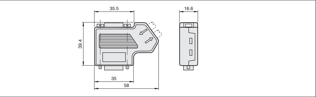
Figure 2.13 Dimensions of the LB9001A
