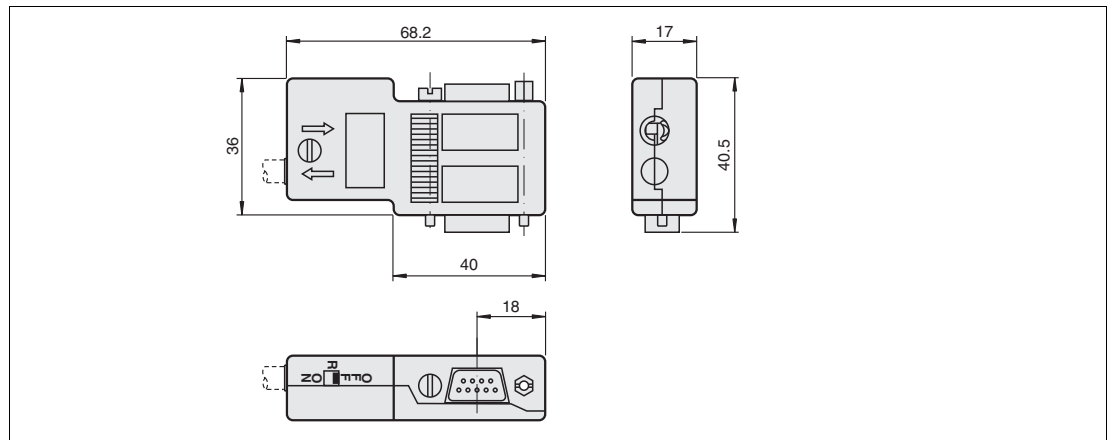
Figure 2.15 Dimensions of the LB9003A
