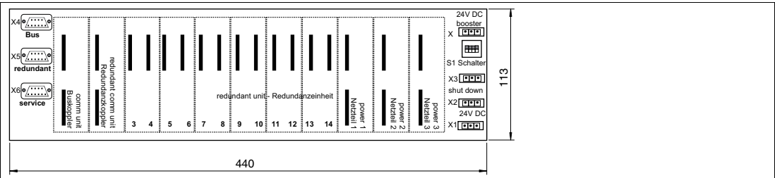
Figure 2.8 Dimensions of the LB9029A
