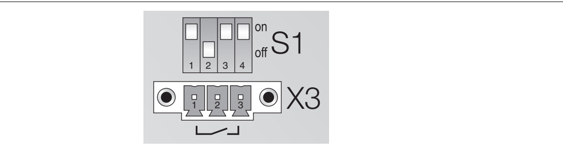
Figure 3.9 X3 terminals and S1 function switches
