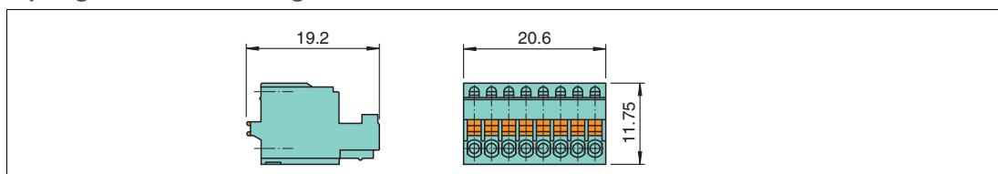
Figure 2.19 Spring terminal dimensions
