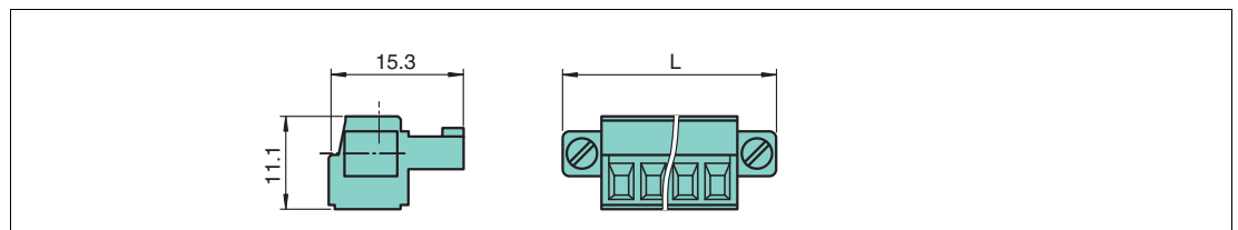
Figure 2.16 Screw terminal dimensions
