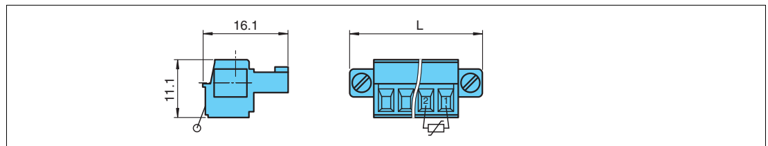
Figure 2.21 Cold junction dimensions L = 33.3 mm for 6-pin terminal
