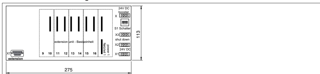
Figure 2.5 Dimensions of the LB9025BP08100.1
