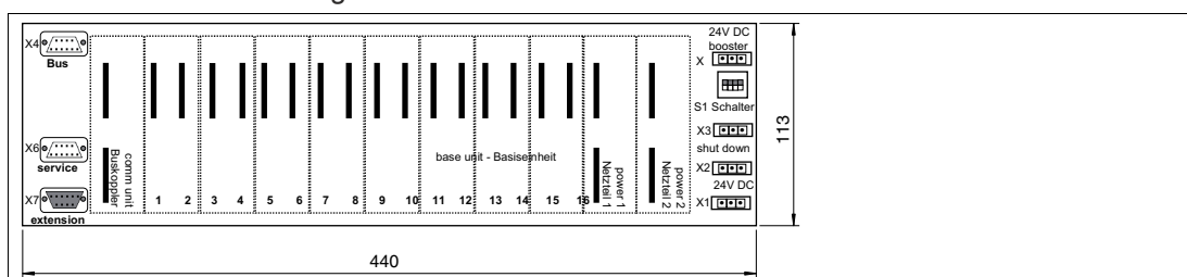
Figure 2.6 Dimensions of the LB9026BP16210.1
