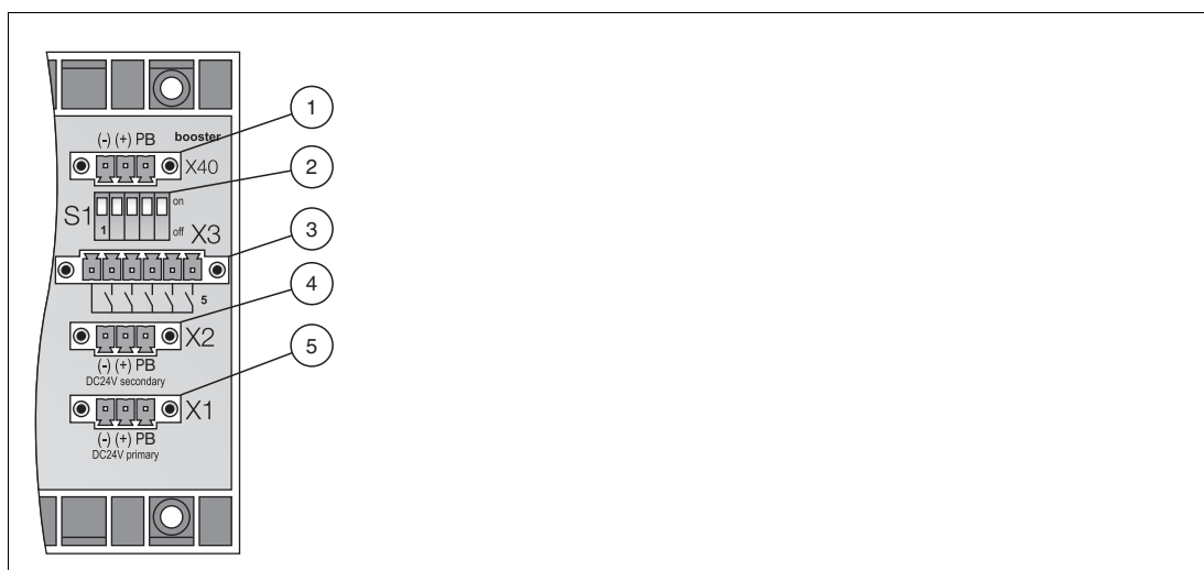
Figure 3.6 Connections on the right-hand side
