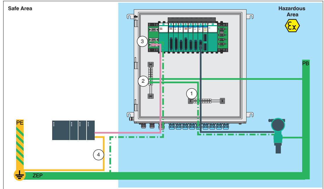
Figure 3.20 Schematic diagram
