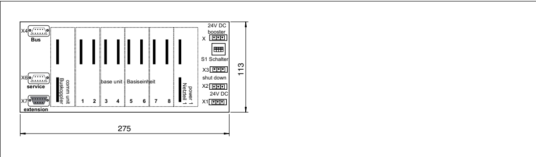
Figure 2.3 Dimensions of the LB9023BP08110.1
