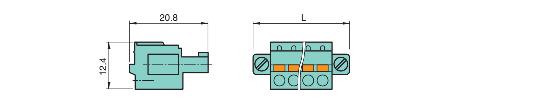
Figure 2.18 Spring terminal dimensions L = 33.3 mm for 6-pin terminal and 40.9 mm for 8-pin terminal
