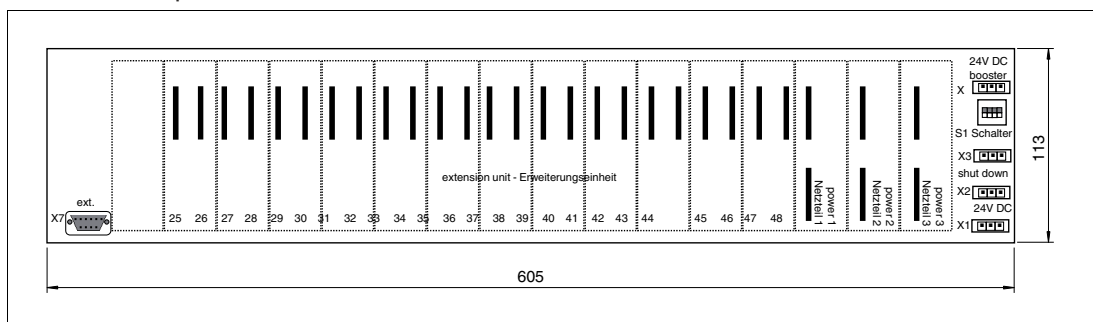
Figure 2.4 Dimensions of the LB9024BP24300.1
