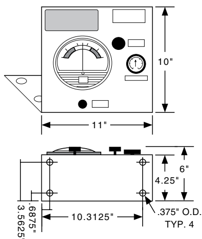
1002-LPS-TM (Top mount configuration)
