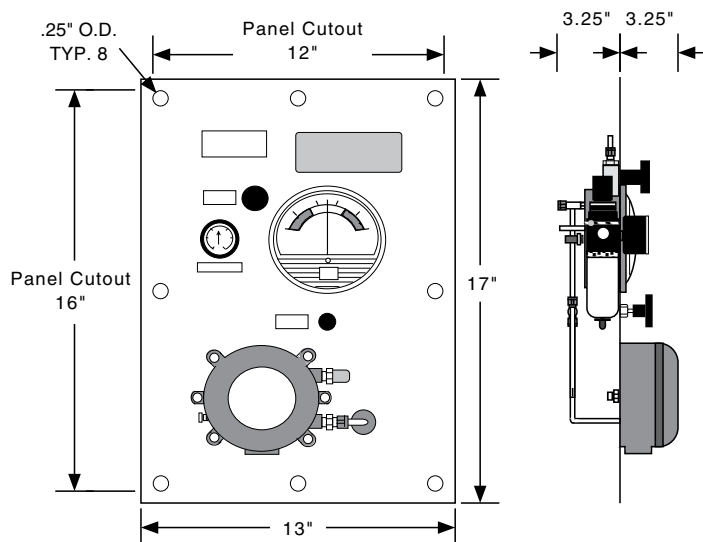
1002-WPS & WPSA-FM (Frame mount configuration)
