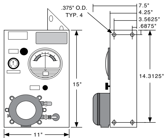
1002-WPS & WPSA-LH (Left hand configuration)
