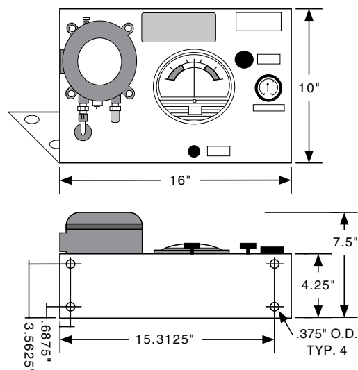
1002-WPS & WPSA-TM (Top mount configuration)
