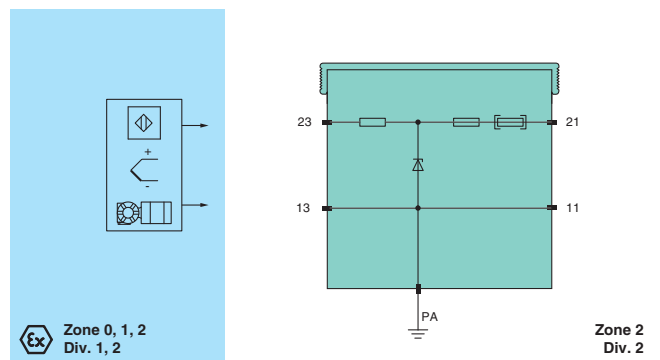
Figure 4 Circuit diagram
