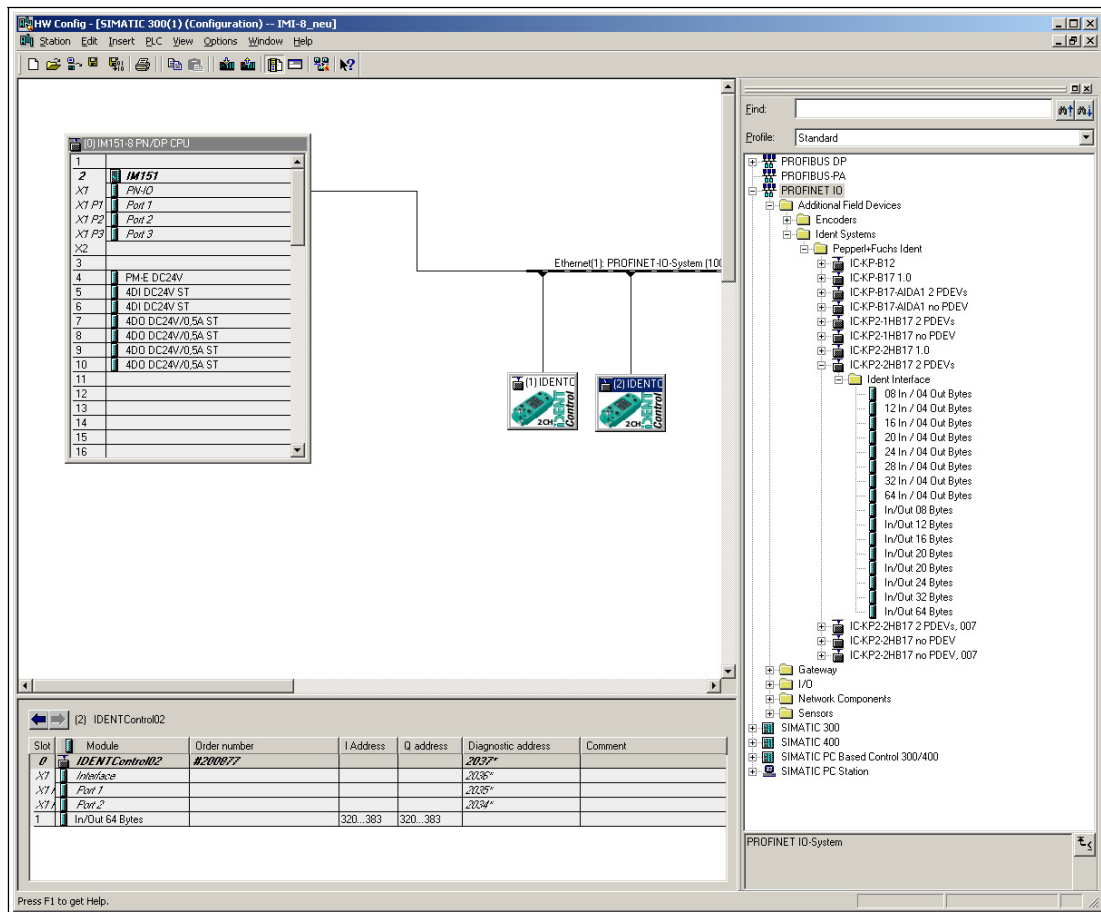
Figure 7.2 HW Konfig / Siemens Step7
