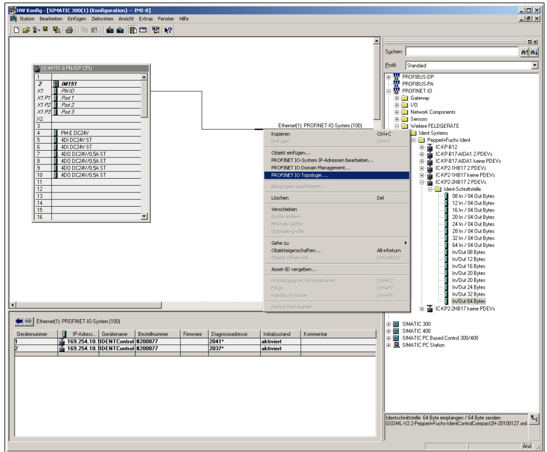
Figure 7.3 Opening the topology editor
