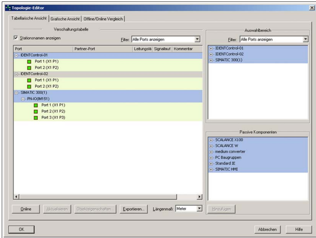
Figure 7.4 Table view
