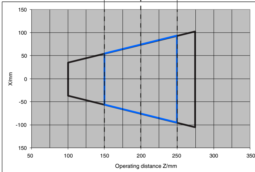
Reading window in X direction
