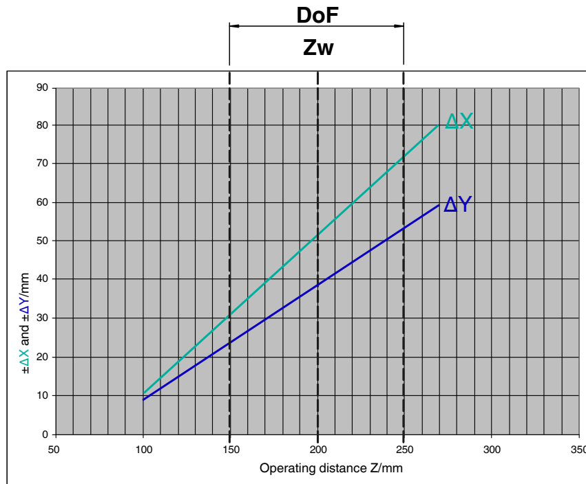
Permissible displacement of read-only tag ( \pm\Delta X and \pm\Delta Y ) depending on reading distance Z
