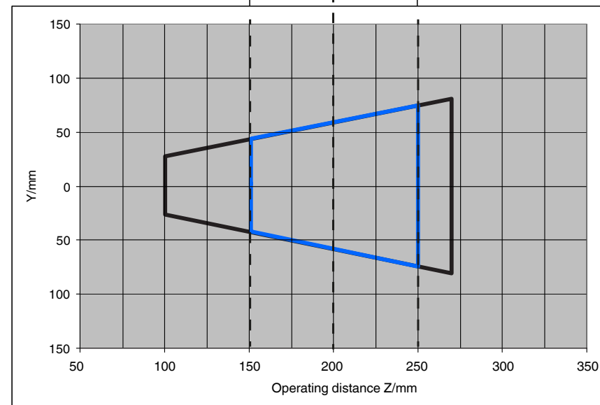
Reading window in Y direction
