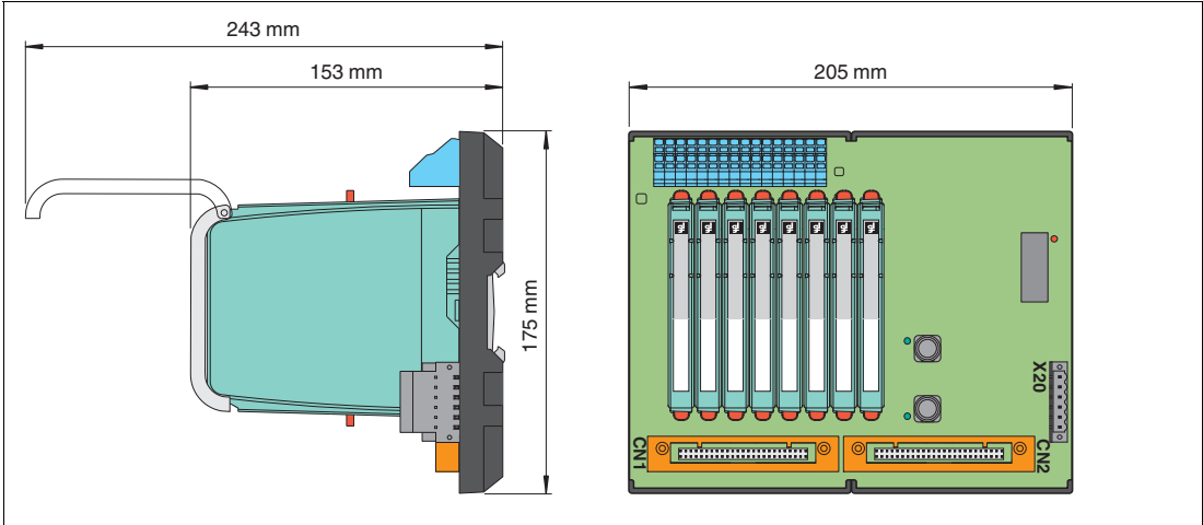
Figure 3.1 Dimensions (W x H x D): 205 x 175 x 153 mm (8.0 x 6.9 x 6.0 inch), depth including module assembly
