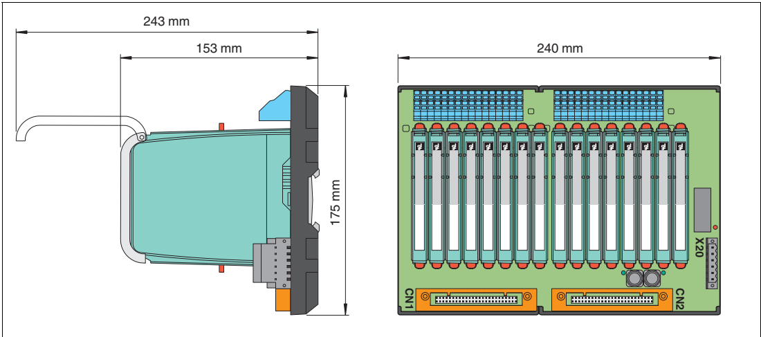
Figure 3.2 Dimensions (W x H x D): 240 x 175 x 153 mm (9.5 x 6.9 x 6.0 inch), depth including module assembly
