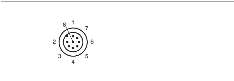
Figure 3.4 Pin assignment receiver unit
