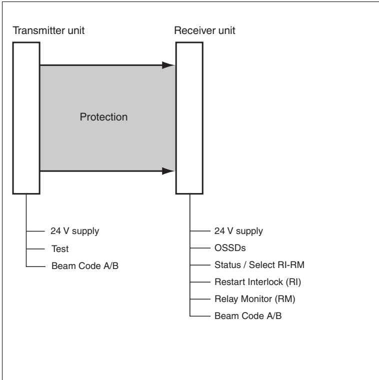
Figure 3.1 Schematic diagram of a detection device
