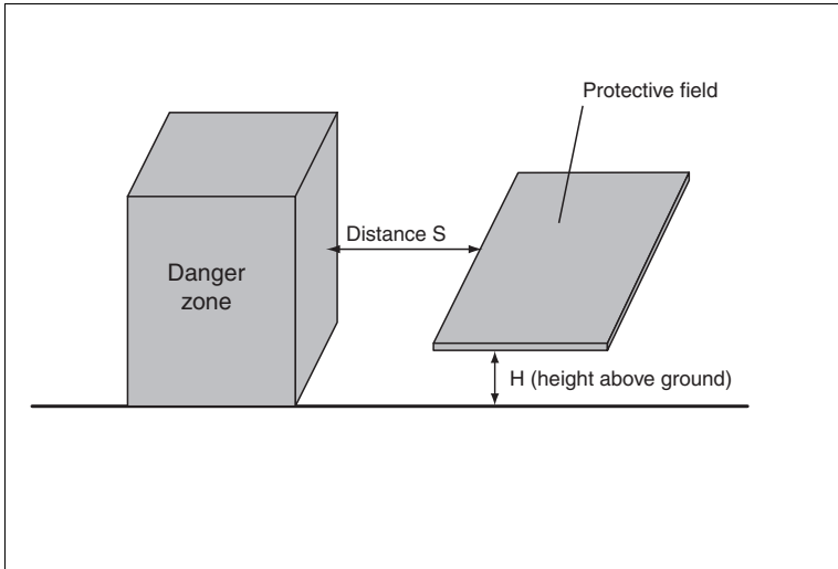
Figure 4.3 Explanation of the safety distance in a horizontal arrangement of the protective field
