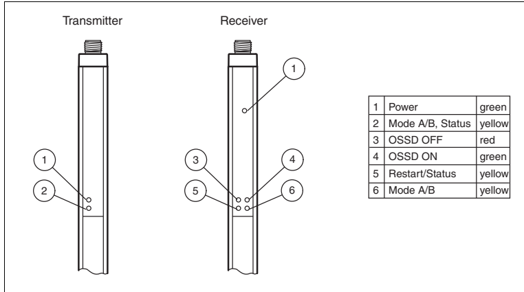
Figure 3.2 Displays on the transmitter and receiver units
