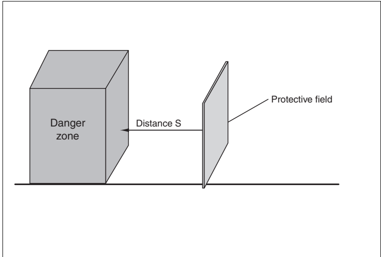
Figure 4.2 Explanation of the safety distance in a vertical arrangement of the protective field
