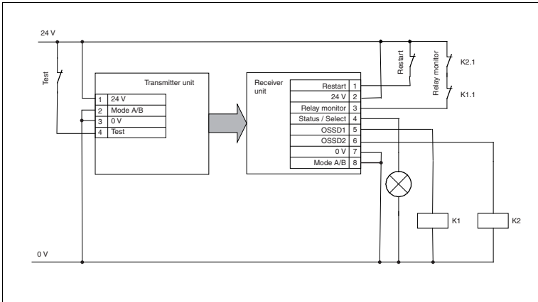
Figure 4.6 Connection example with relay monitor and restart in Mode A
