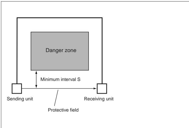
Figure 4.1 Minimum distance between protection field and hazardous area
