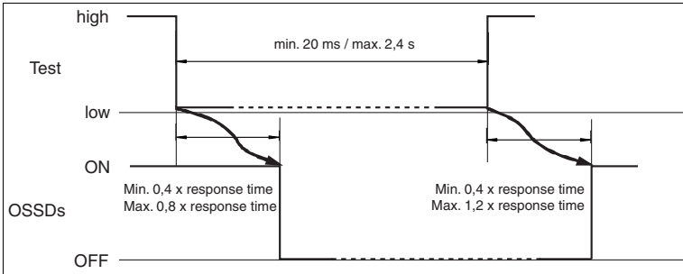
Figure 4.5 Graphs of the OSSD switching states when initiating a test or reset
