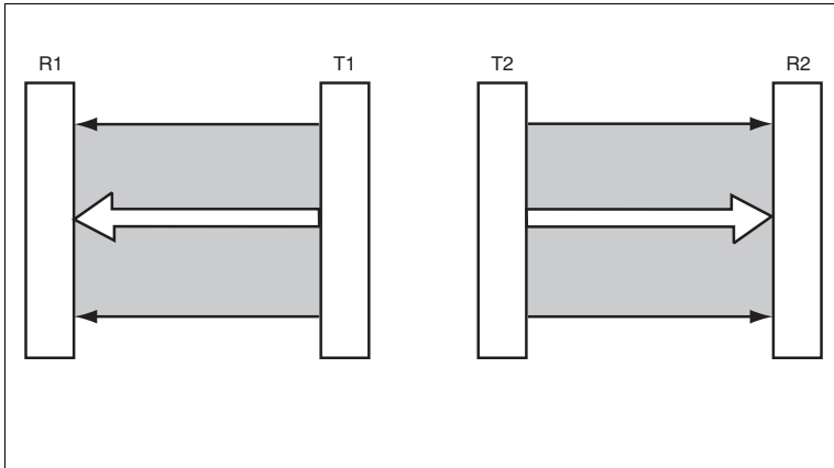
Figure 5.1 Multiple assignment
