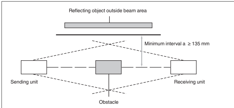
Figure 4.4 Explanation to the risk of radiation protection of remirroring
