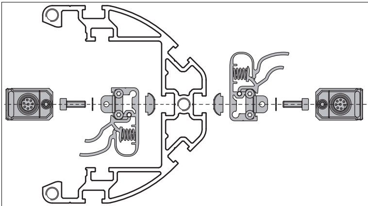
Figure 8.5 Example of mounting a mounting aid OMH-SLCT-01 to a mounting column
