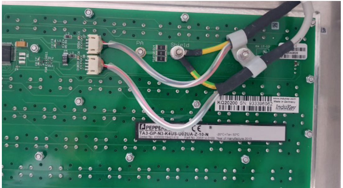
Figure 3.4 Tighten the protective earth to a torque of 0.15 Nm. Tighten the cable clamp to a torque of 0.3 Nm.
