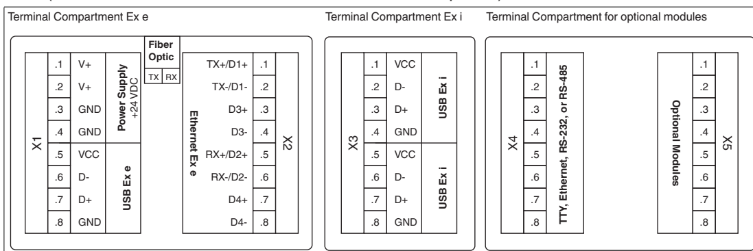
Figure 3.3 Terminal compartments
