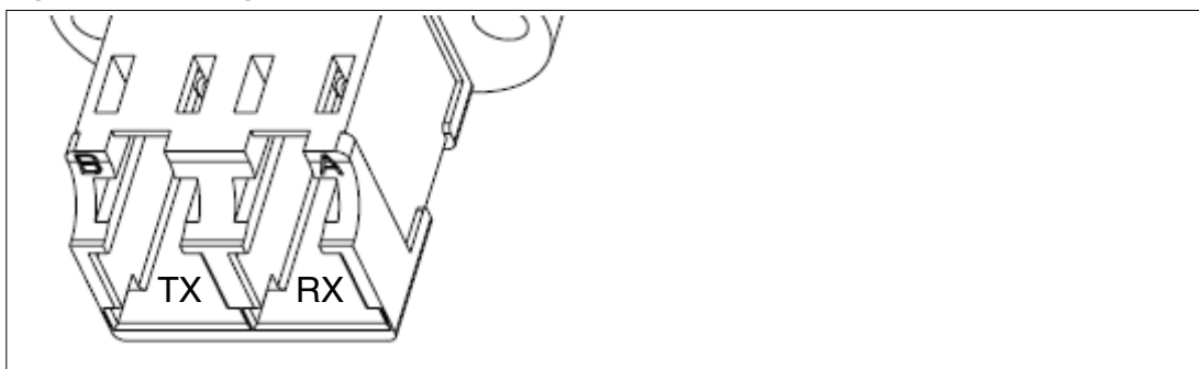
Figure 3.4 For the optional Fiber optic interface a duplex LC connection is required.
