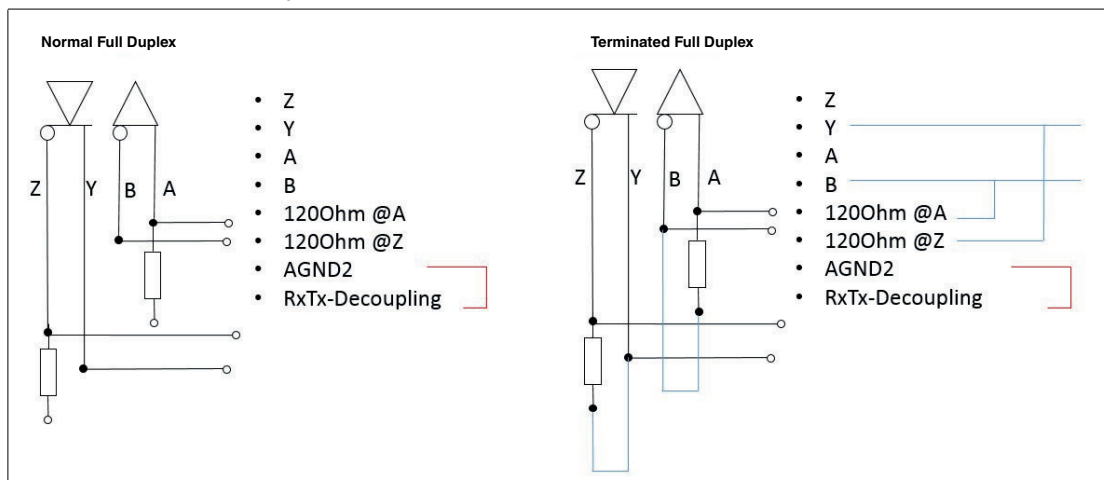
Figure 3.8 Full duplex cabling
