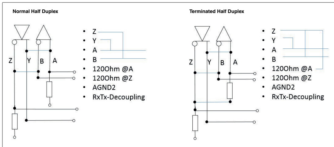
Figure 3.9 Half duplex cabling
