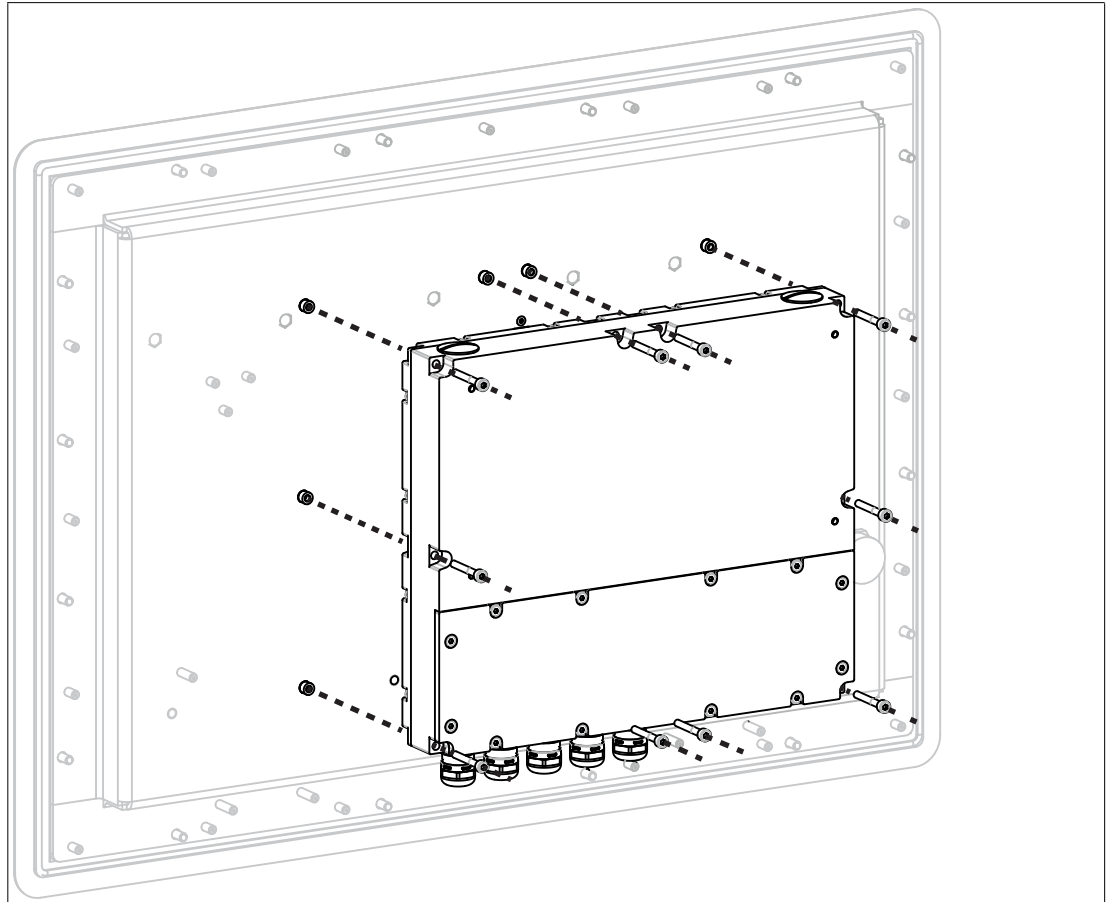
Figure 3.11 Mounting the TCU/PCU onto the display unit
