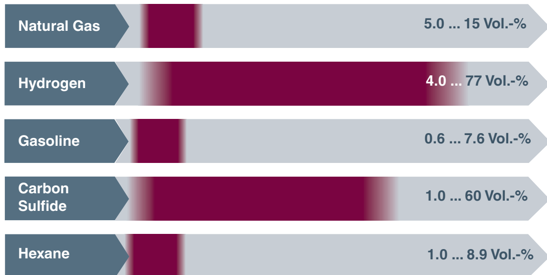
Figure 8. Explosive limits of selected gases and vapors
