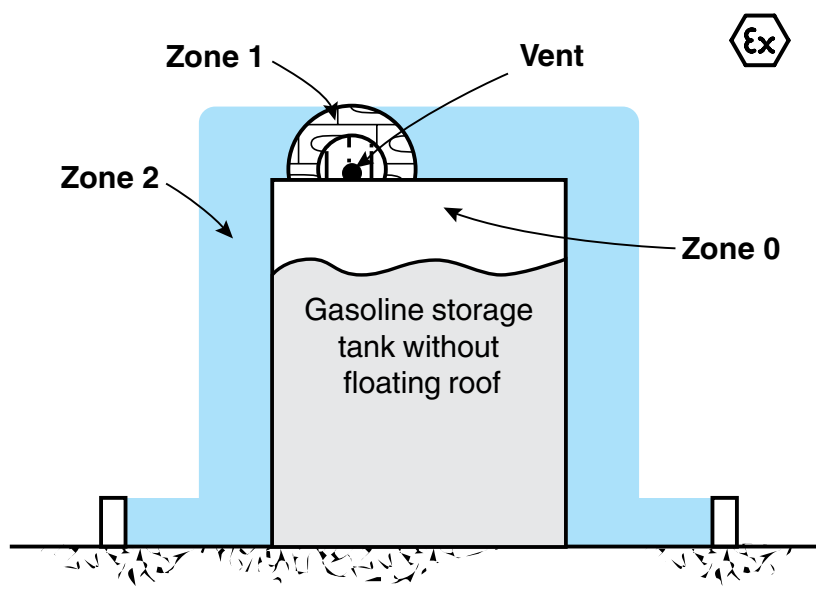
Figure 4. Schematic view of how the surroundings of a fuel tank with a fixed roof and vent are divided into different zones
