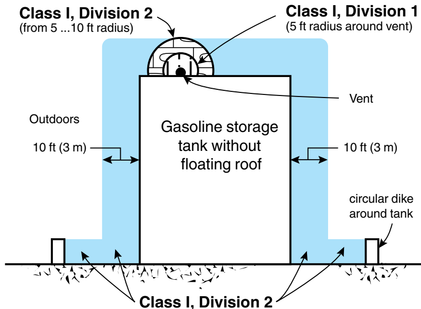
Figure 5. Schematic of a division-based area classification of a gasoline storage tank with fixed lid and breather.
