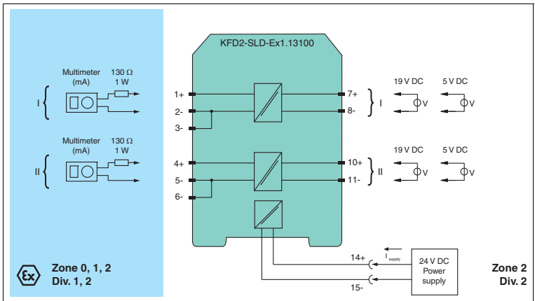
Figure 5.1 Proof test set-up for KFD2-SLD-Ex1.13100
