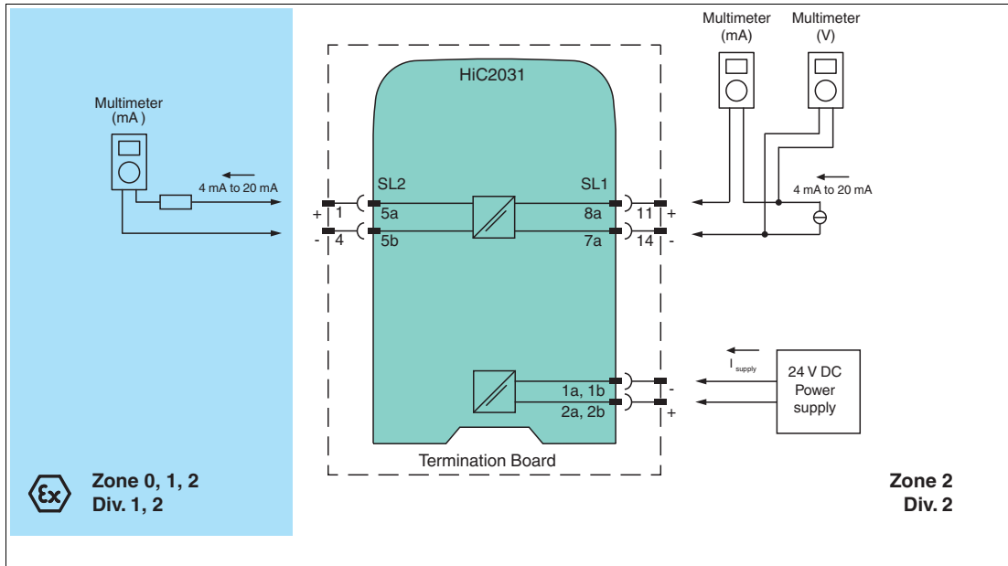
Figure 5.2 Proof test set-up for HiC2031
