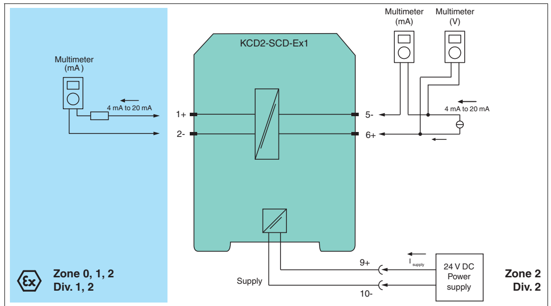
Figure 5.1 Proof test set-up for KCD2-SCD-(Ex)1(.SP)
