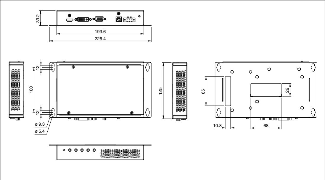
Figure 3.4 Dimensions
