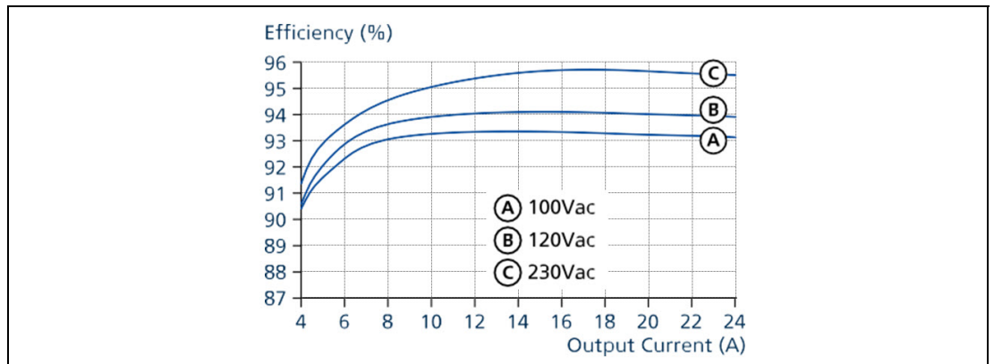
Figure 11.1 Efficiency vs. output current at 24V, typ.
