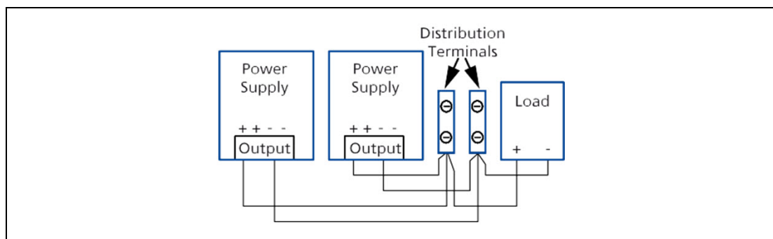
Figure 14.1 Using distribution terminals
