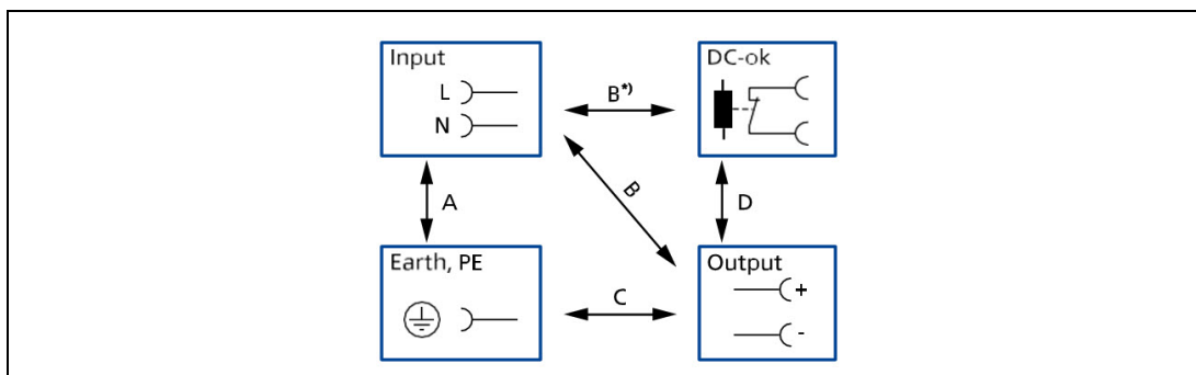
Figure 21.1 Dielectric strength
