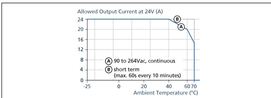
Figure 18.1 Output current vs. ambient temp.
