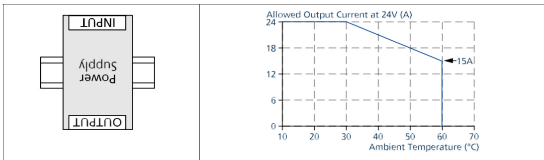
Figure 26.11 Mounting orientation B (upside down)
