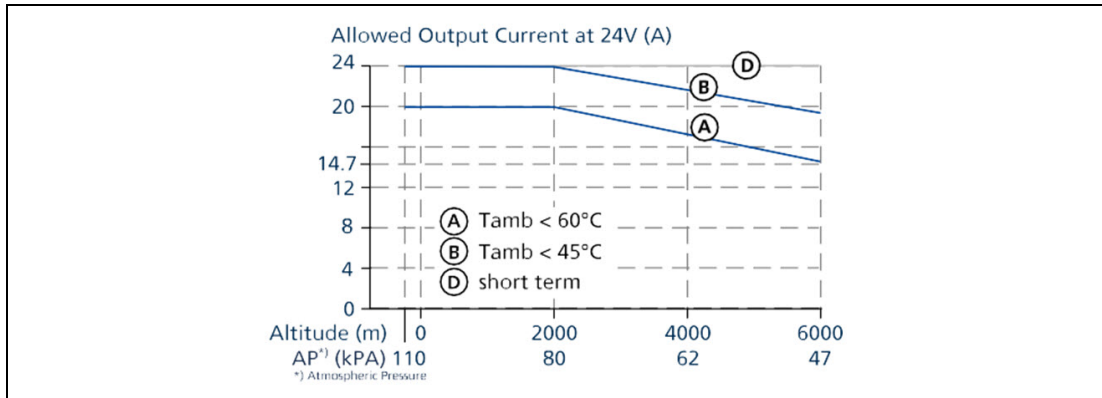
Figure 18.2 Output current vs. altitude
