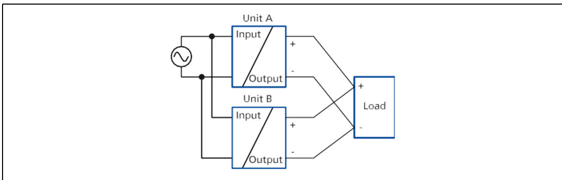
Figure 26.6 Parallel use to increase output power
