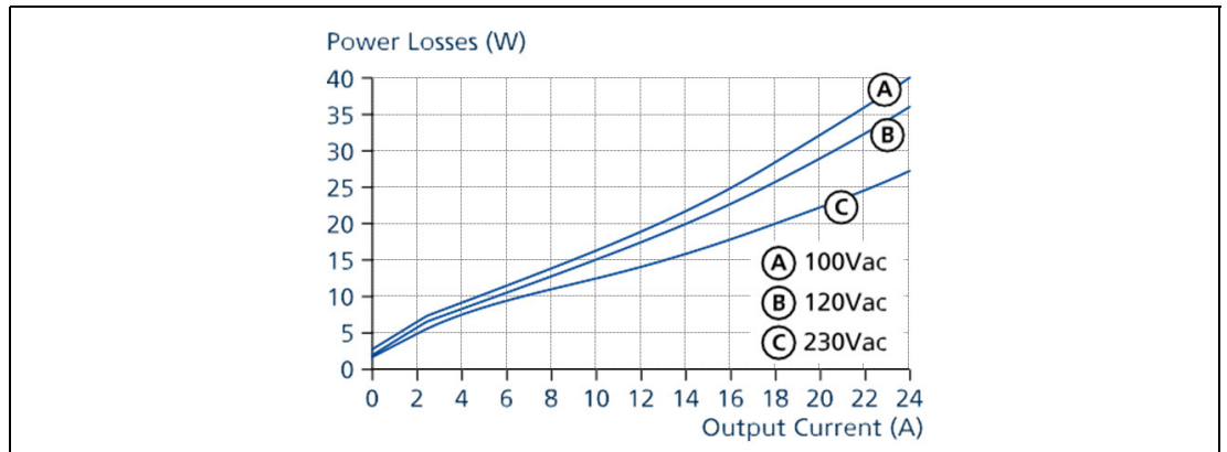
Figure 11.2 Losses vs. output current at 24V, typ.
