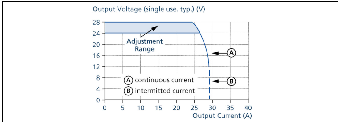
Figure 8.1 Output voltage vs. output current, typ.
