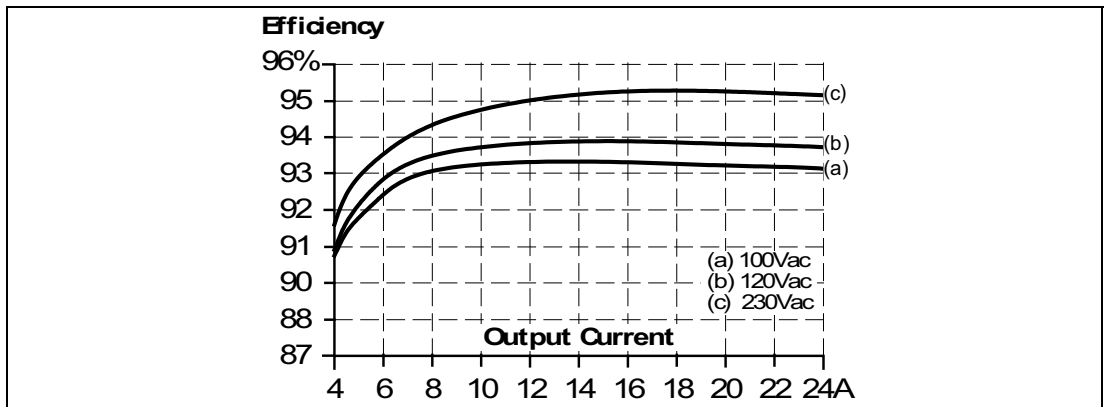
Figure 11.1 Efficiency vs. output current, typ.
