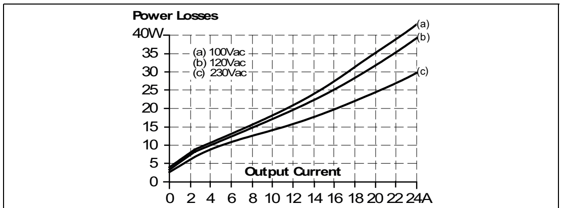
Figure 11.2 Losses vs. output current, typ.
