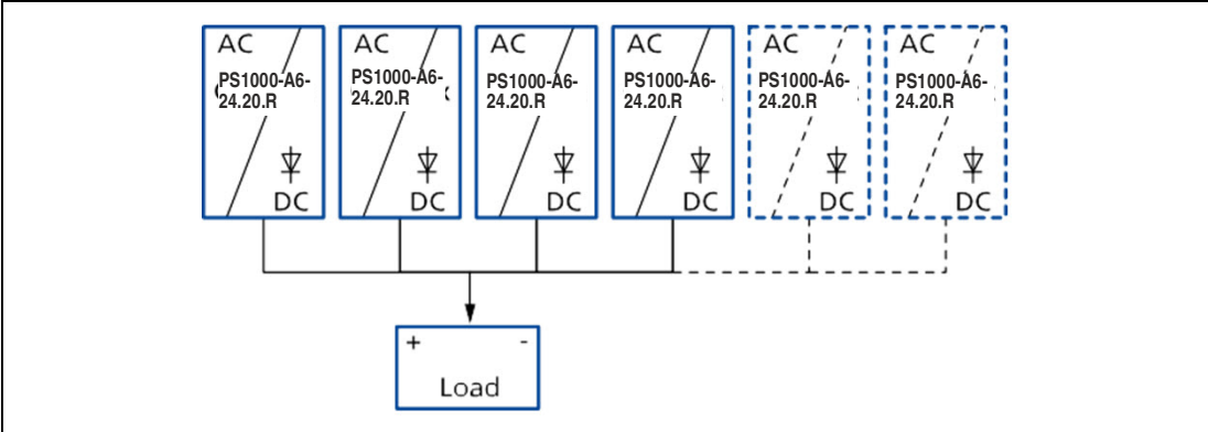
Figure 2.2 N+1 Redundancy
