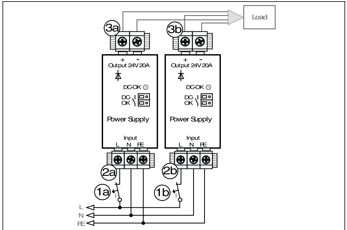
Figure 16.1 Replacing the device or redundancy module while the system is running
