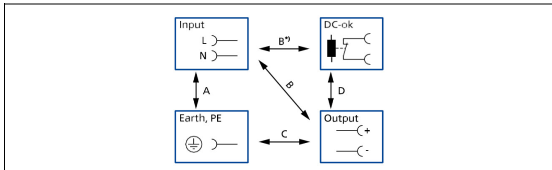
Figure 21.1 Dielectric strength
