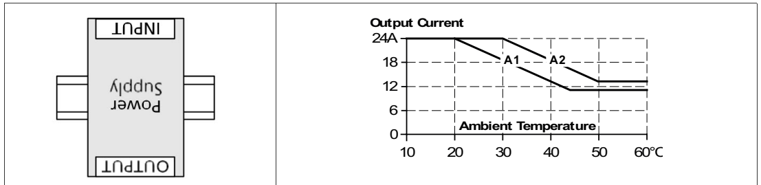
Figure 25.14 Mounting orientation B (upside down)
