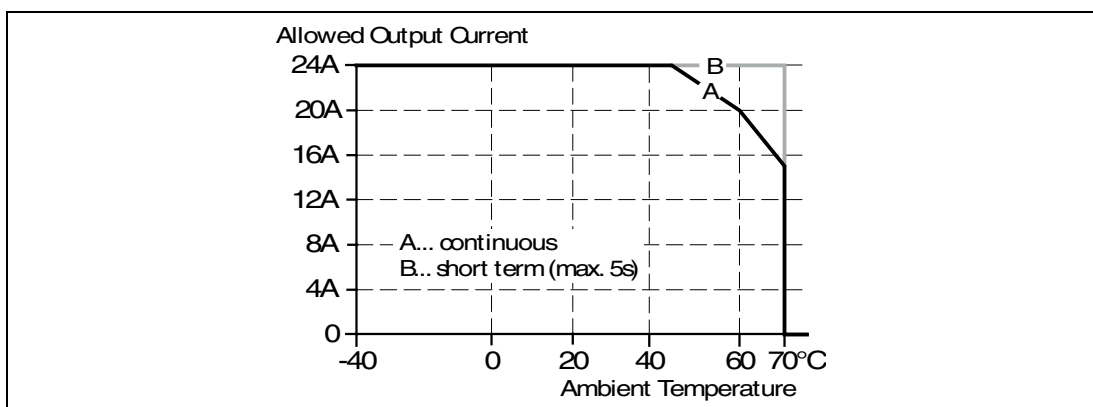
Figure 19.1 Output current vs. ambient temperature (I nom 20A; I out with PowerBoost = 24A)
