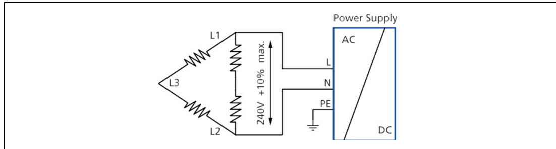
Figure 25.12 Operation on two phases
