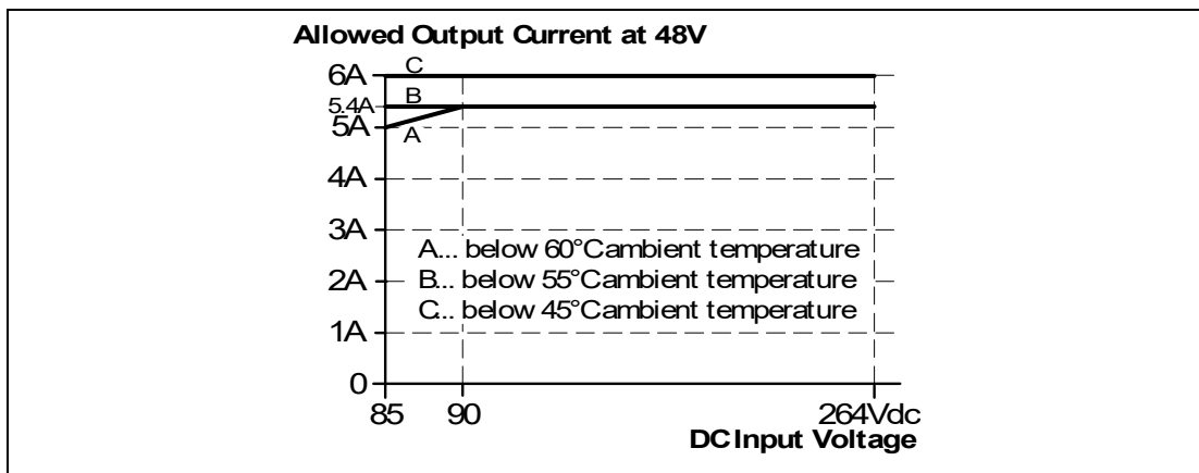
Figure 5.5 Derating requirements
