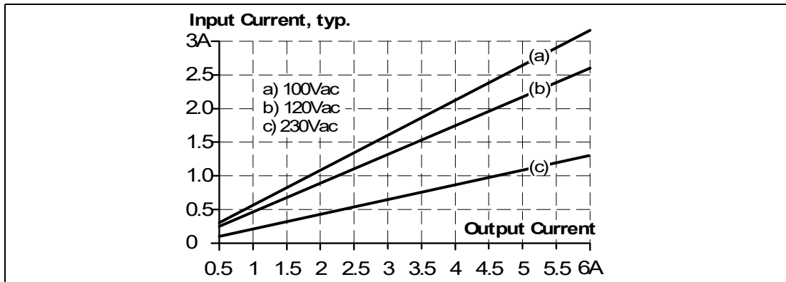
Figure 5.3 Input current vs. output current at 48V output voltage
