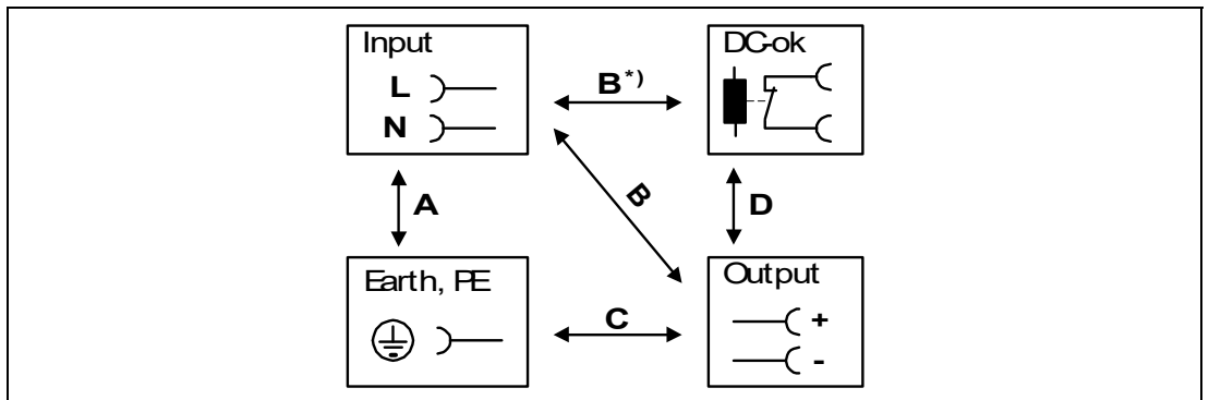
Figure 21.1 Dielectric strength
