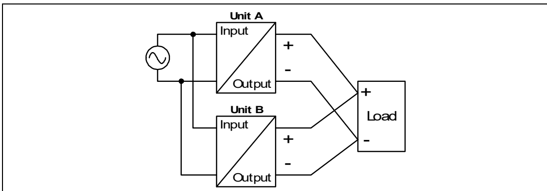
Figure 25.5 Parallel use to increase output power
