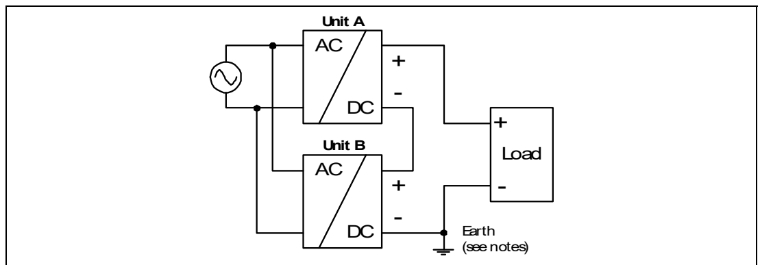
Figure 25.6 Series operation
