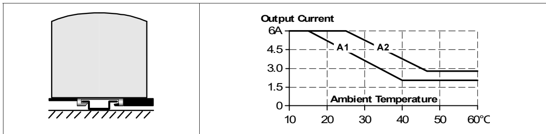
Figure 25.10 Mounting orientation C (table-top mounting)
