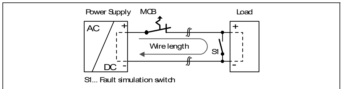
Figure 25.4 Test circuit
