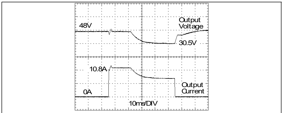
Figure 25.1 10.8A peak current for 50ms , typ. (2x the nominal current)
