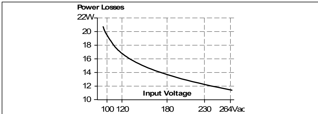
Figure 11.4 Losses vs. input voltage at 48V, 5.4A, typ.
