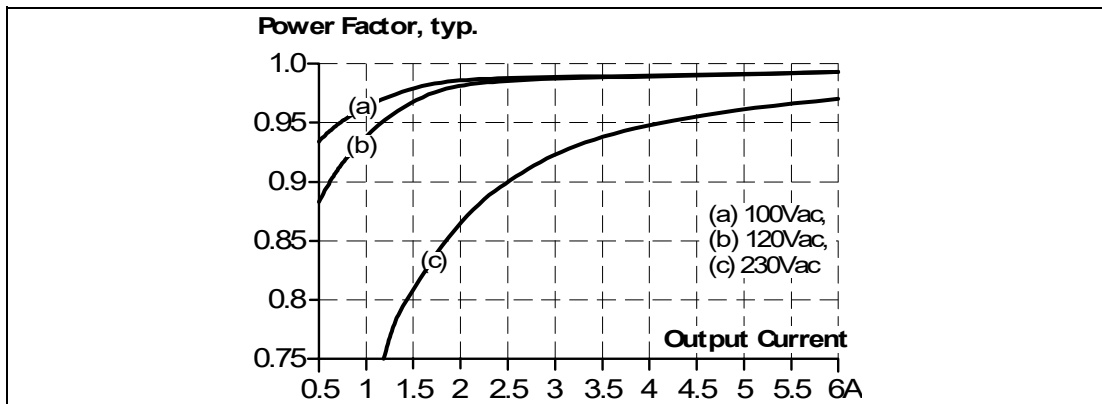
Figure 5.4 Power factor vs. output current at 48V output voltage
