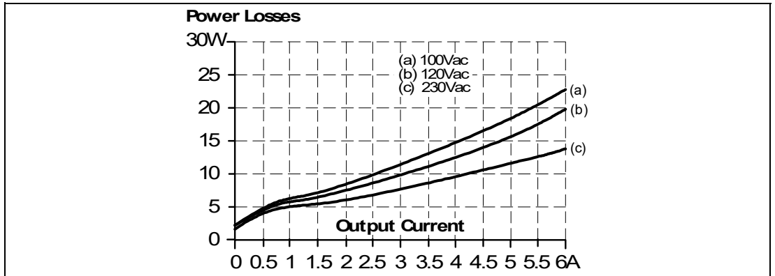
Figure 11.2 Losses vs. output current at 48V, typ.
