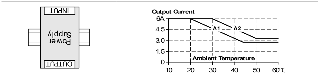
Figure 25.9 Mounting orientation B (upside down)
