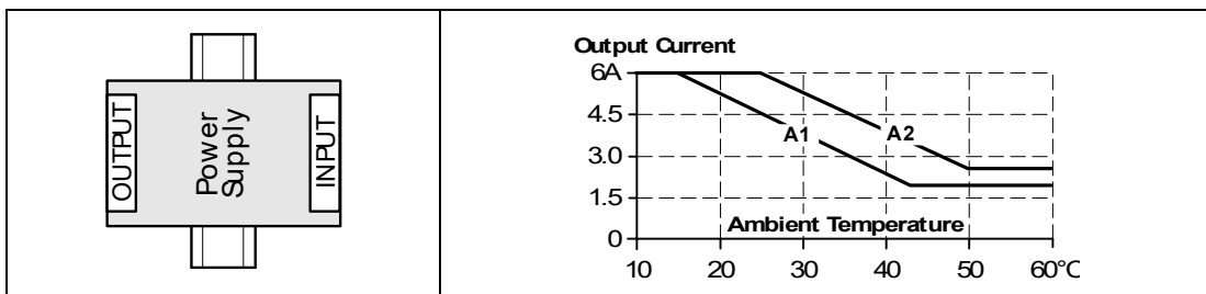
Figure 25.12 Mounting orientation E (horizontal ccw)
