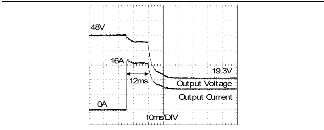
Figure 25.3 16A peak current for 12ms , typ. (3x the nominal current)
