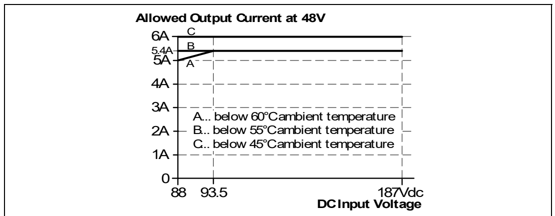
Figure 6.2 Derating requirements
