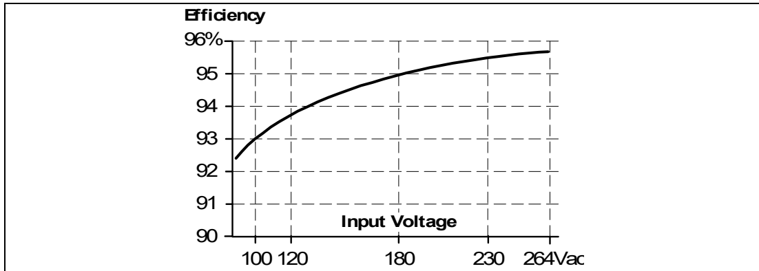
Figure 11.3 Efficiency vs. input voltage at 48V, 5.4A, typ.
