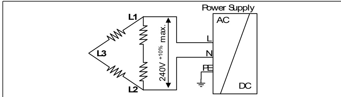
Figure 25.7 Two phases operation
