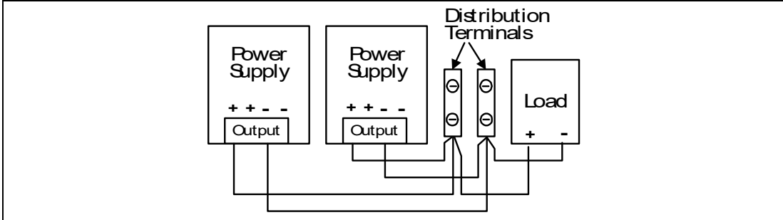
Figure 15.2 Using distribution terminals
