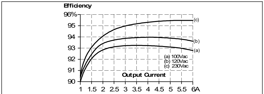
Figure 11.1 Efficiency vs. output current at 48V, typ.
