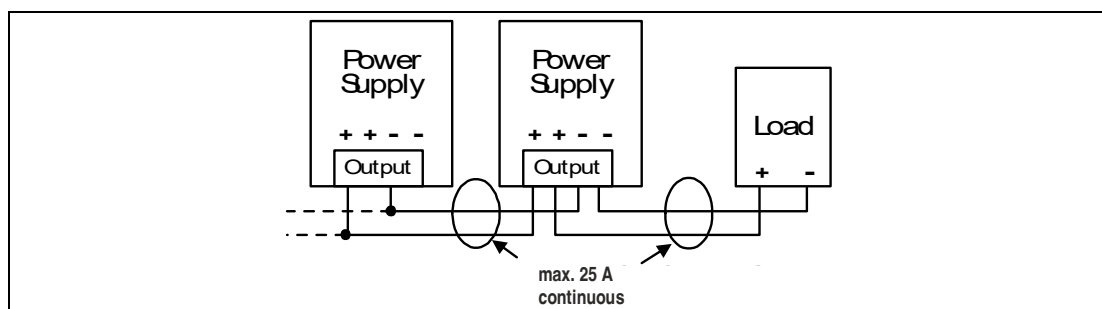
Figure 15.1 Daisy chaining of outputs
