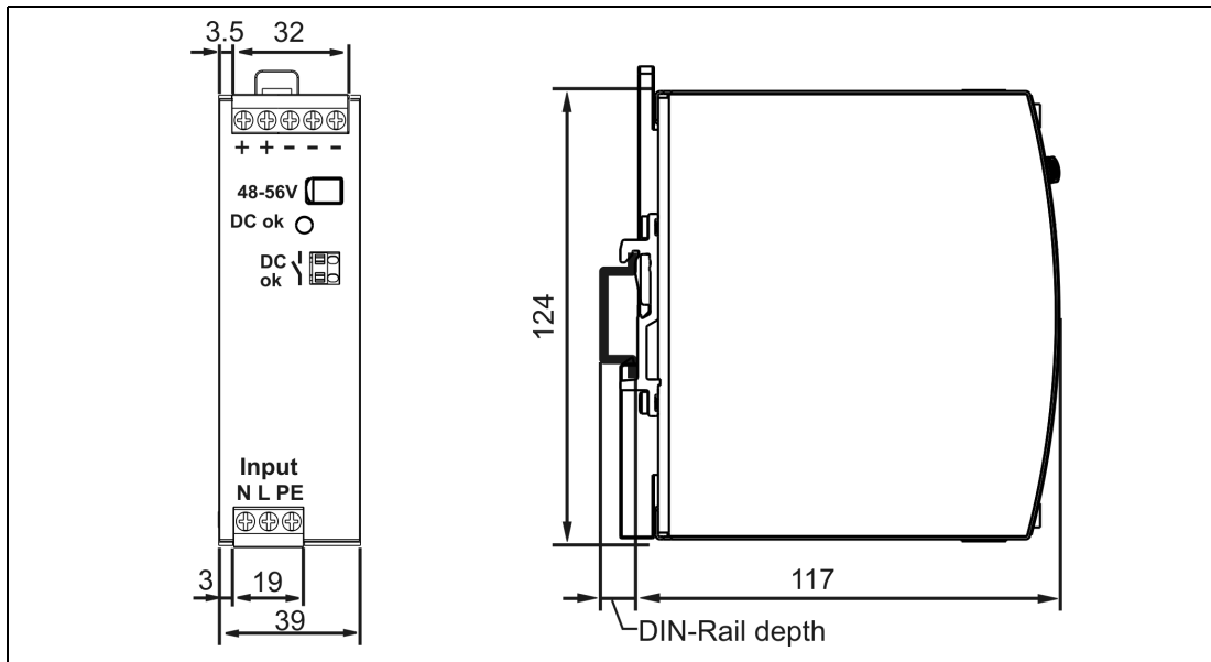
Figure 24.1 Device dimensions, all dimensions in mm
