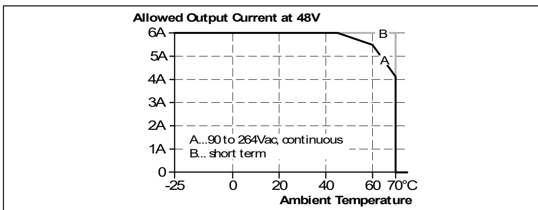
Figure 18.1 Output current vs. ambient temp.
