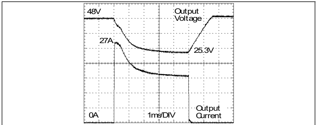
Figure 25.2 27A peak current for 5ms , typ. (5x the nominal current)
