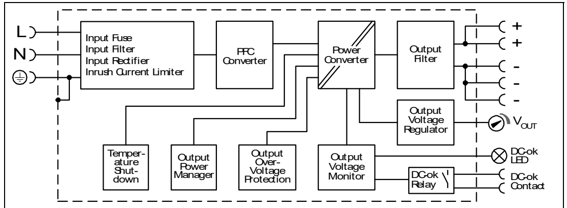
Figure 14.1 Functional diagram
