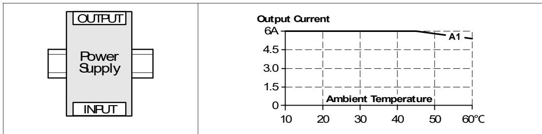
Figure 25.8 Mounting orientation A (standard orientation)
