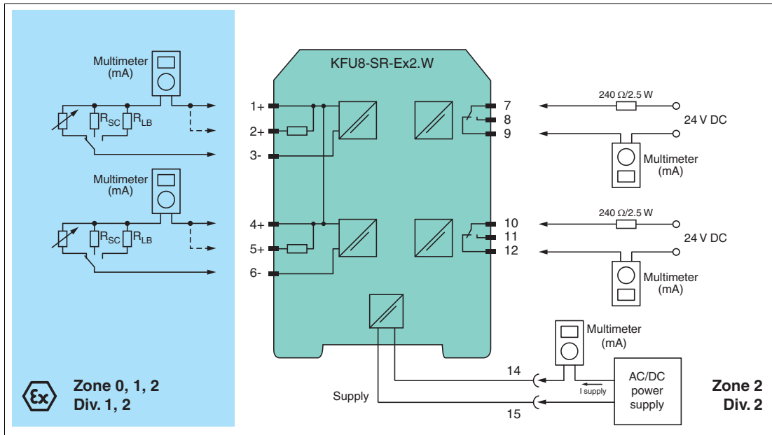
Figure 5.3 Proof test set-up for KFU8-SR-Ex2.W
