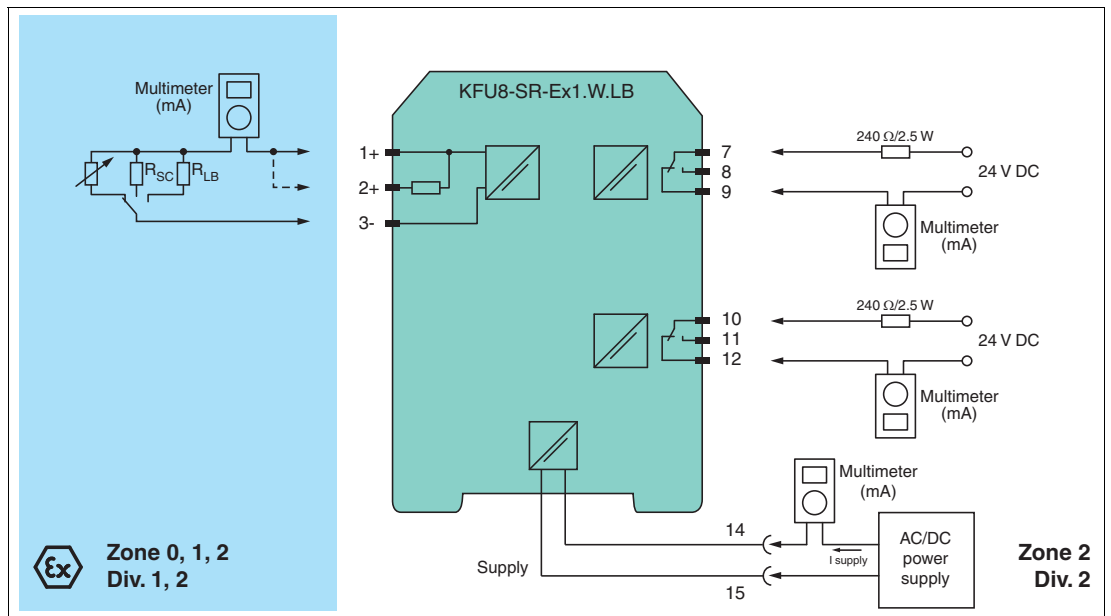
Figure 5.2 Proof test set-up for KFU8-SR-Ex1.W.LB
