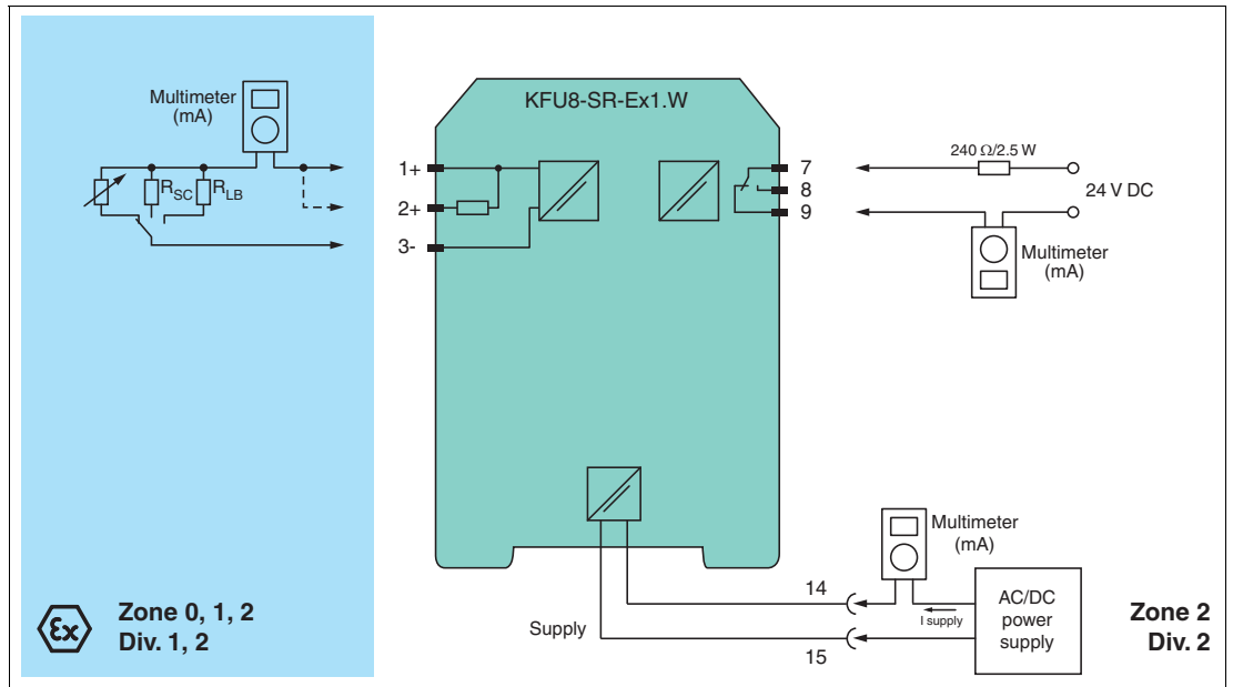
Figure 5.1 Proof test set-up for KFU8-SR-Ex1.W
