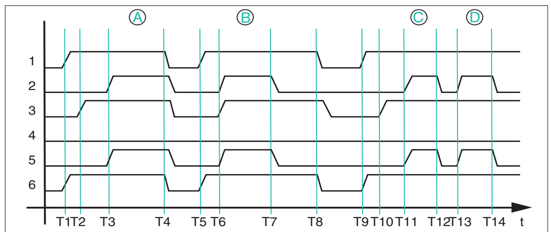
Figure 7.3 Timing sequence of bits in byte 0
