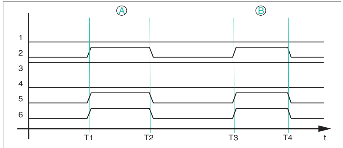
Figure 7.2 Timing sequence of bits in byte 0
