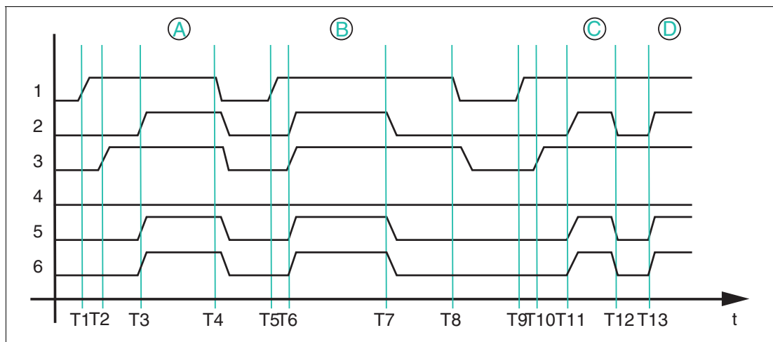
Figure 7.1 Timing sequence of bits in byte 0
