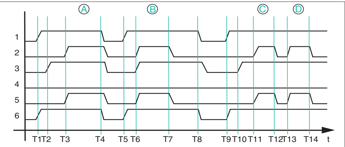
Figure 7.3 Timing sequence of bits in byte 0
