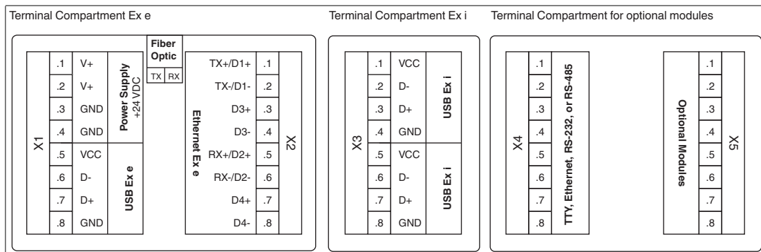
Figure 4.3 Terminal compartments
