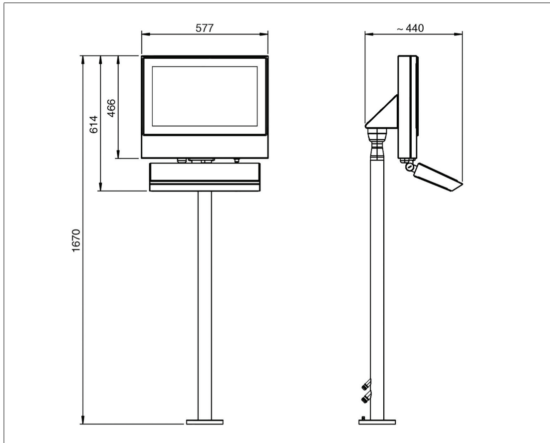
Figure 3.5 0° tilted with pedestal or wall mounting
