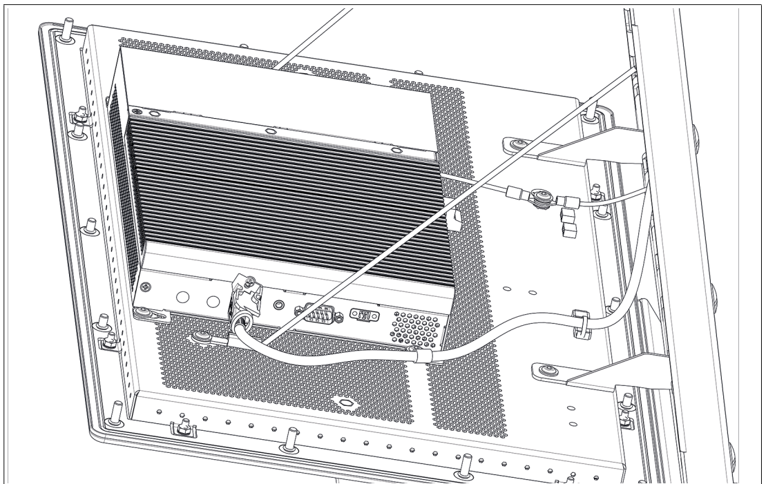
Figure 7.20 Cable routing without configured RFID reader
