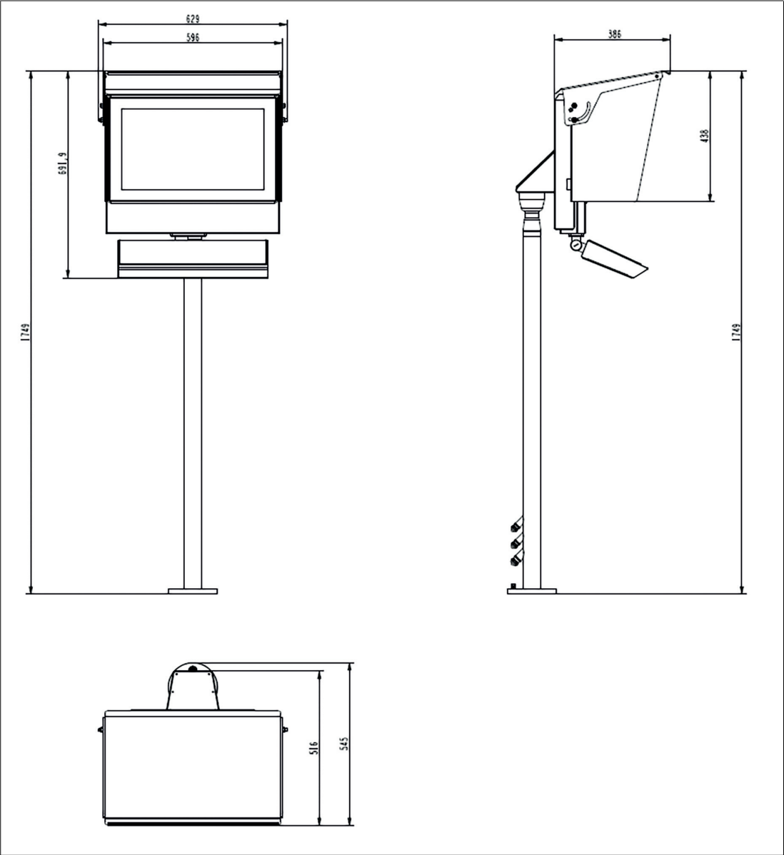
Figure 3.6 0° tilted with pedestal, Dimensions with Top, Sides, Back shields
