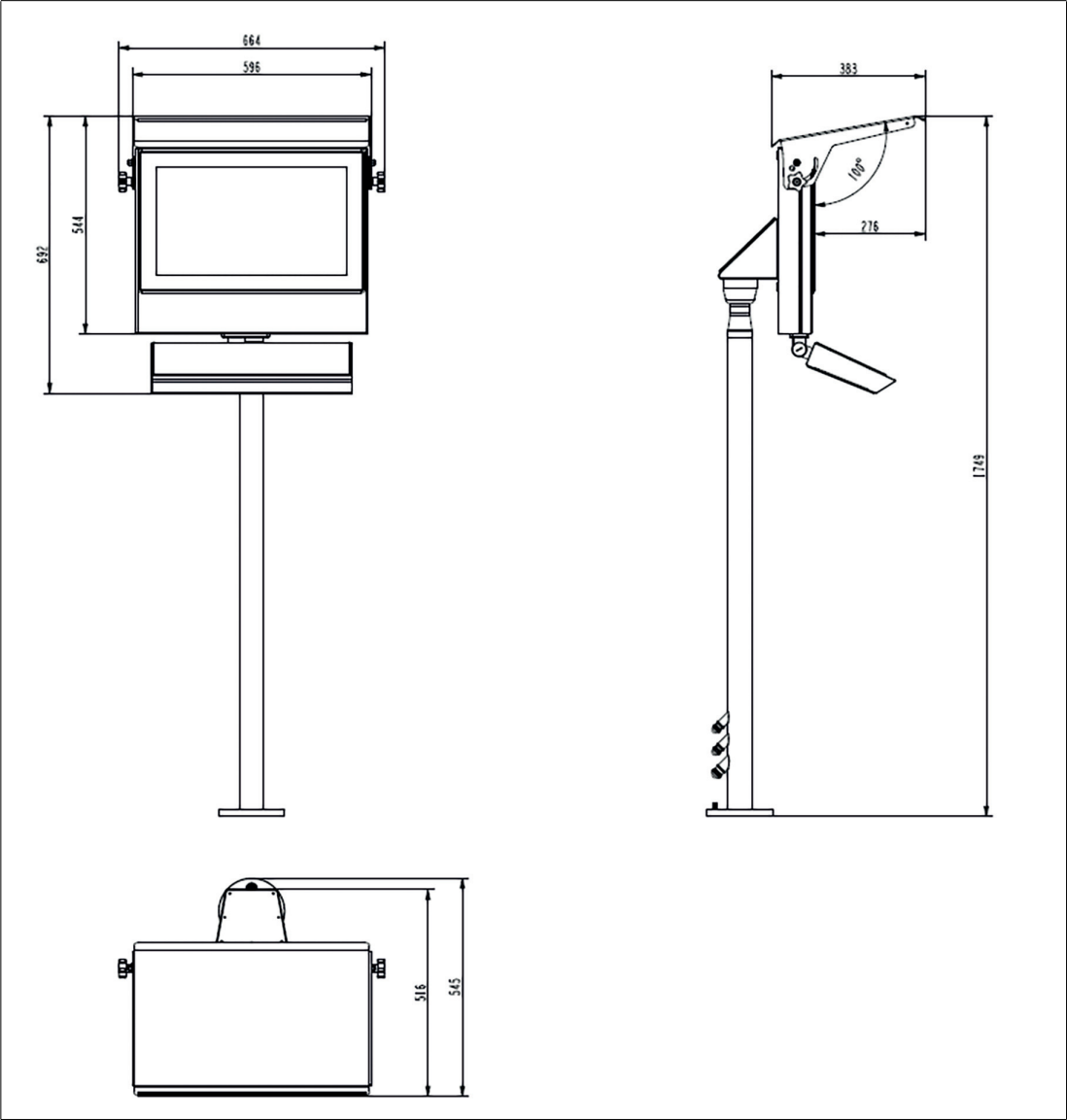
Figure 3.7 0° tilted with pedestal, Dimensions with Top and Back shields
