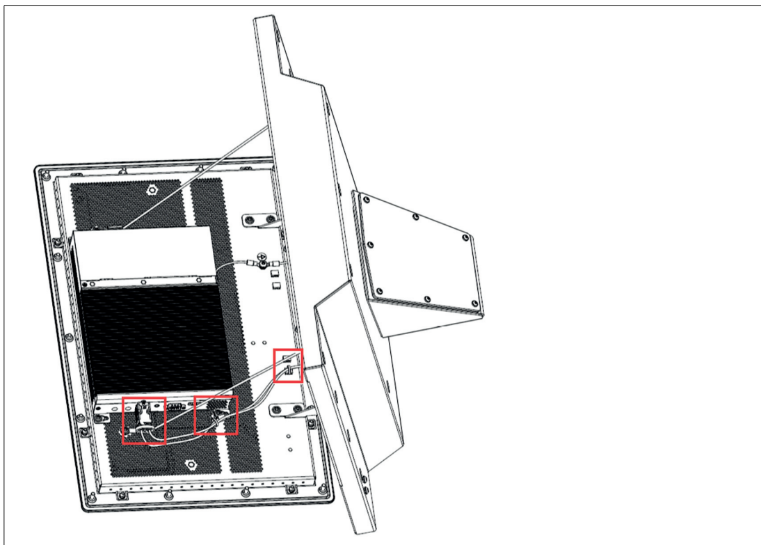
Figure 7.21 Cable routing with configured RFID reader
