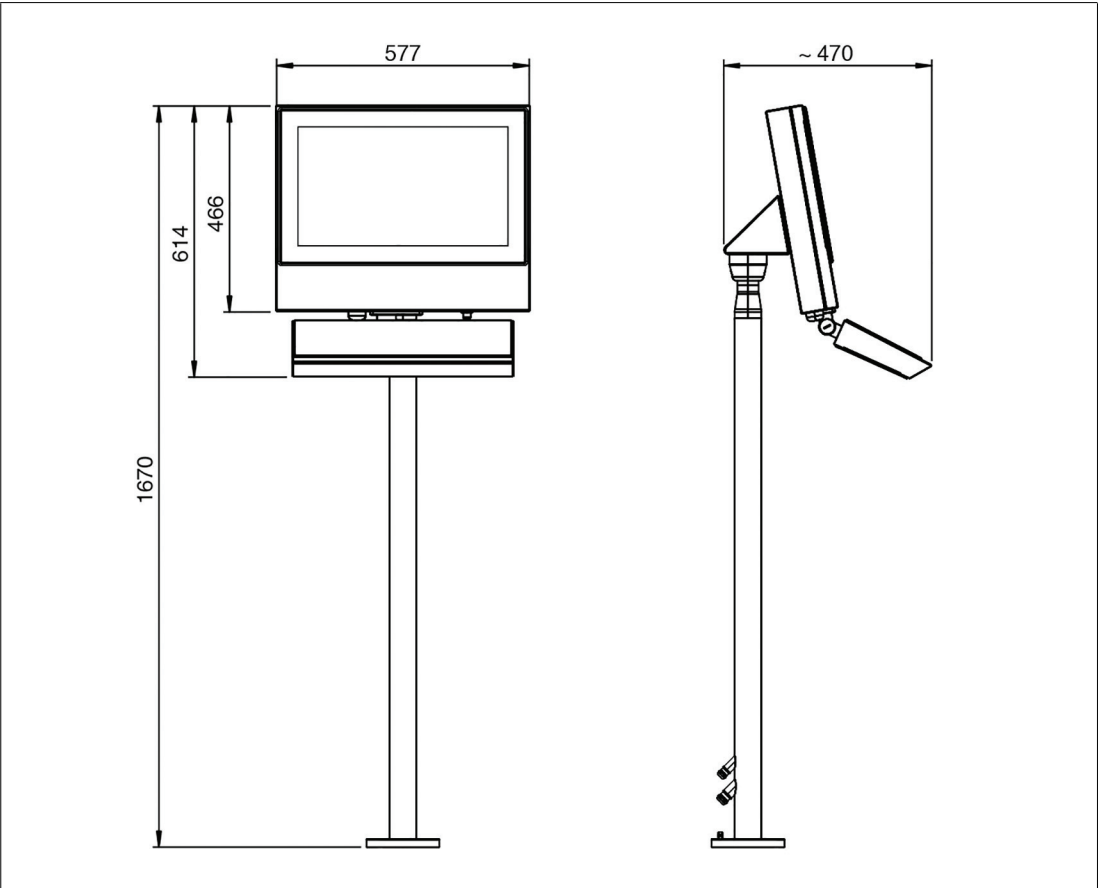
Figure 3.4 10° tilted system with pedestal
