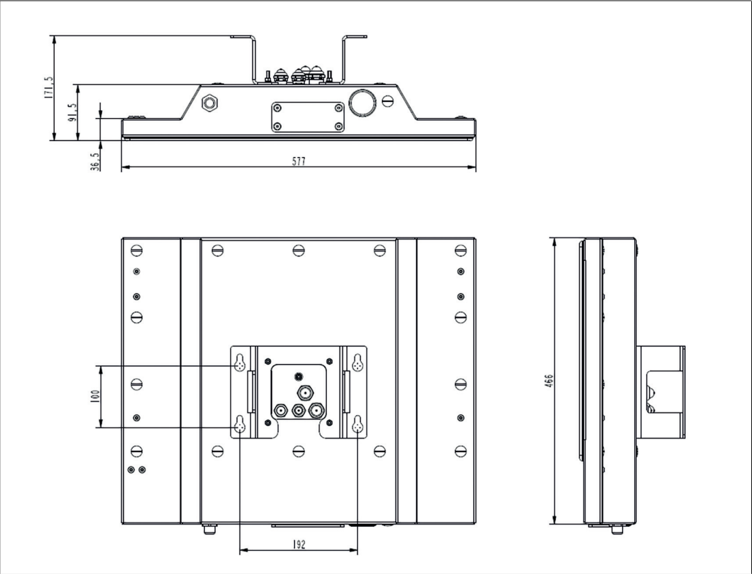
Figure 3.8 Dimensions Wall Mounting
