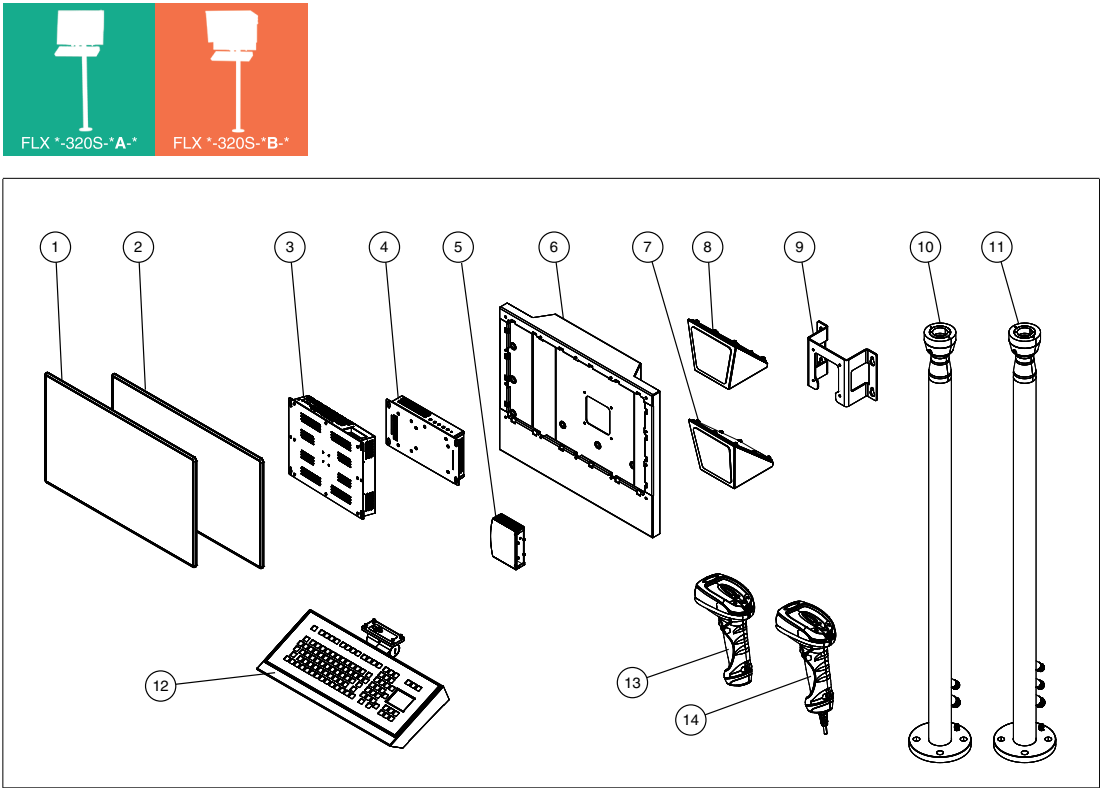
Figure 11.1 VisuNet FLX System - possible configurations
