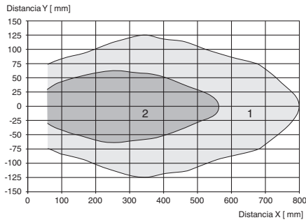
Curva 1: placa plana 100 mm x 100 mm Curva 2: barra redonda, Ø 25 mm
