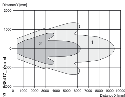
Distance Y [mm] Distance X [mm] Courbe 1: surface unie 100 mm x 100 mm Courbe 2: barre ronde, Ø 25 mm
