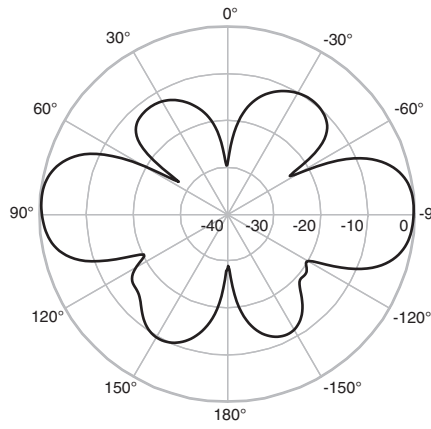
vertical 2.4 GHz
