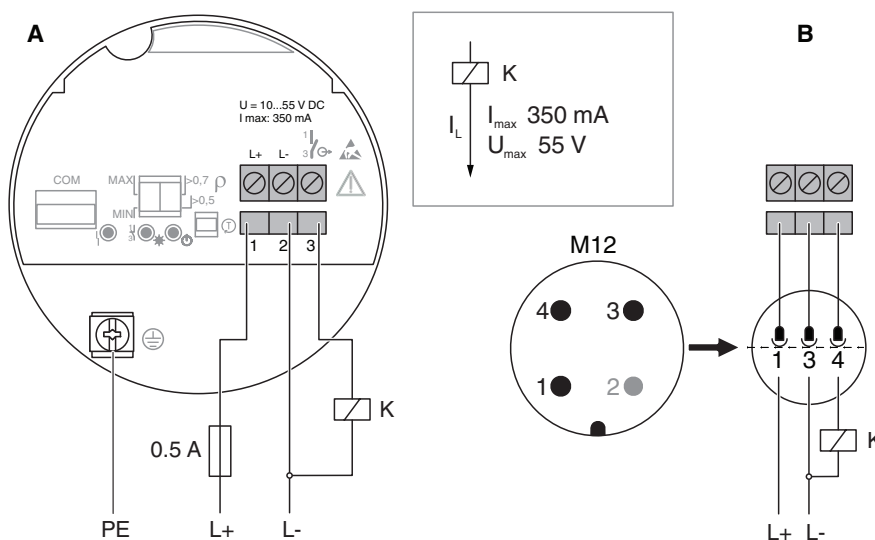
3-wire DC-PNP, electronic insert FEL62 (example)
