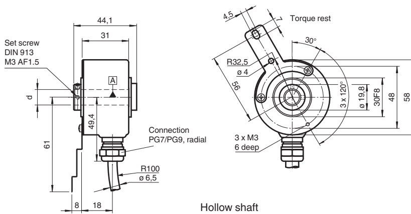
Hollow shaft
